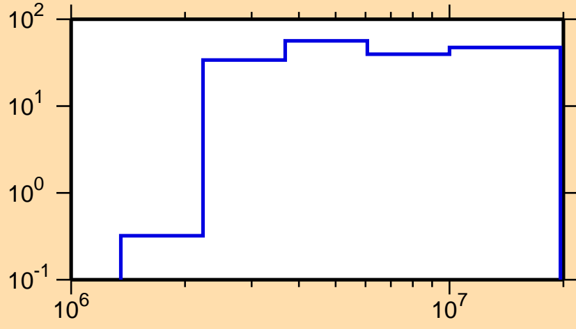
\Delta\sigma/\sigma vs. E for ^{209}\text{Bi}(n,p)
