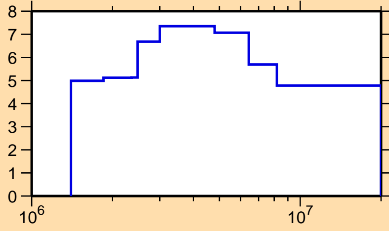
\Delta\sigma/\sigma vs. E for ^{209}\text{Bi}(n,el.)
