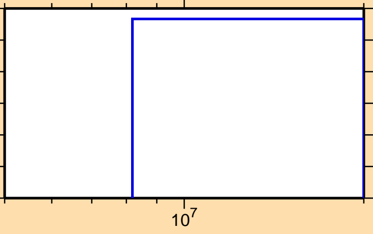
\sigma vs. E for ^{209}\text{Bi}(n,nt)
