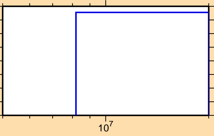
\sigma vs. E for ^{210}\text{Bi}(n,\text{nd})
