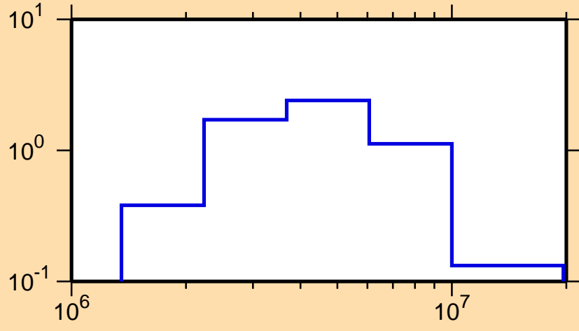
\sigma vs. E for ^{211}\text{Bi}(n,n\text{cont.})
