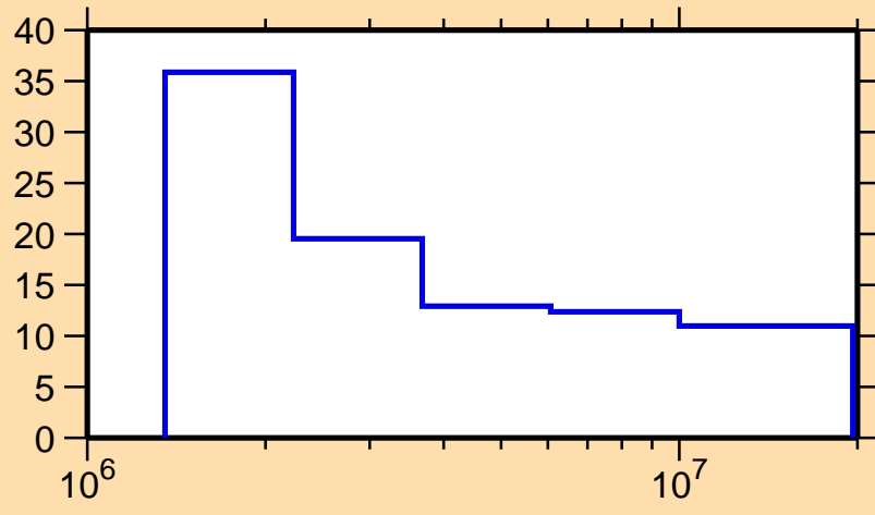
\Delta\sigma/\sigma vs. E for ^{211}\text{Bi}(n,n\text{nonel.})
