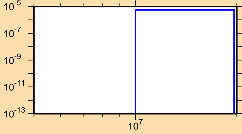
\sigma vs. E for ^{211}\text{Bi}(n,nd)
