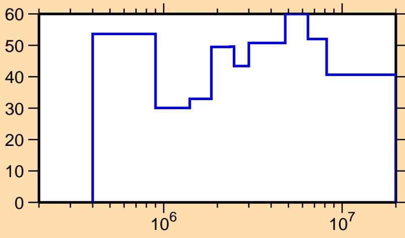
\Delta\sigma/\sigma vs. E for ^{211}\text{Bi}(n,n_1)
