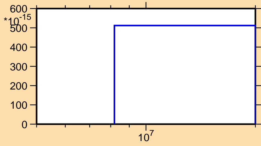
\sigma vs. E for ^{211}\text{Bi}(n,\text{He3})
