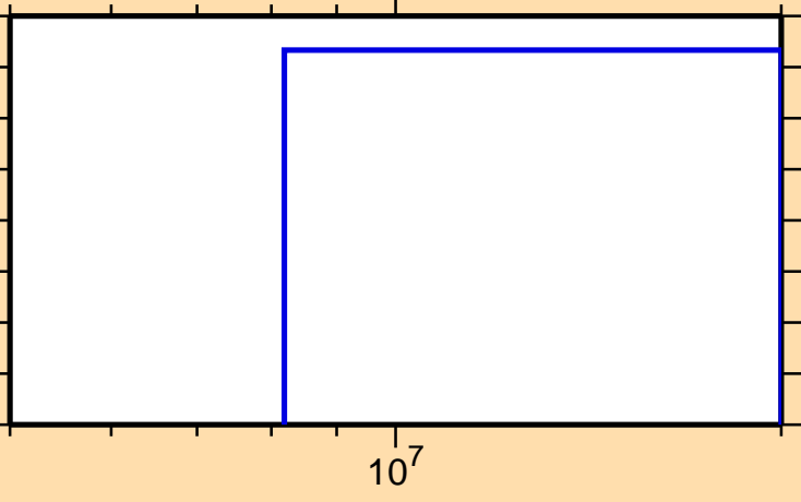
\sigma vs. E for ^{211}\text{Bi}(n,nt)
