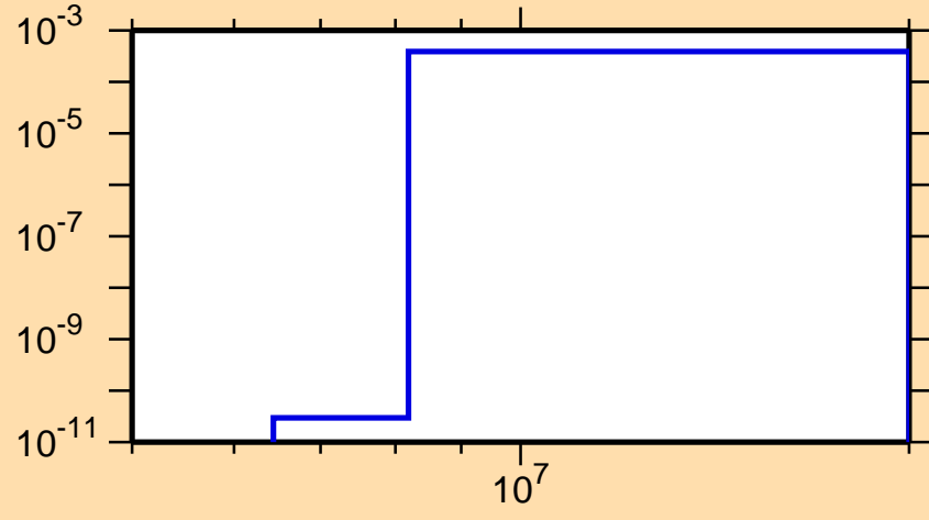
\sigma vs. E for ^{211}\text{Bi}(n,np)
