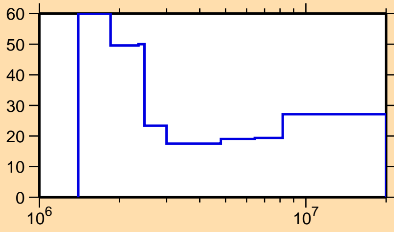
\Delta\sigma/\sigma vs. E for ^{211}\text{Bi}(n,n\text{cont.})
