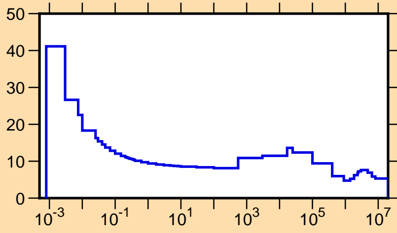
\sigma vs. E for ^{212}\text{Bi}(n,\text{tot.})
