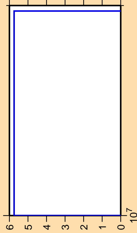
\Delta\sigma/\sigma vs. E for ^{212}\text{Bi} (mt 45)
