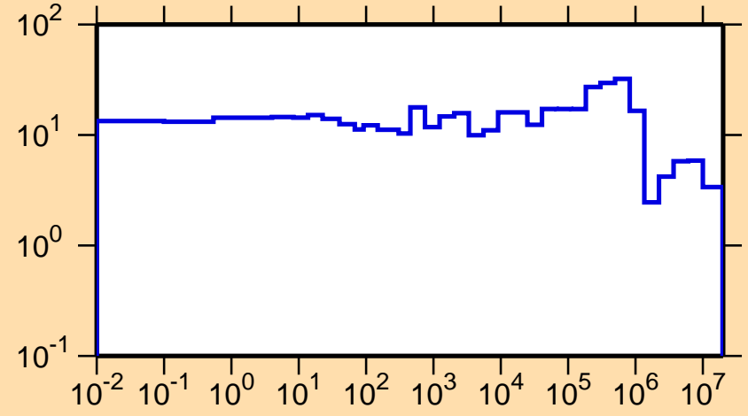
\Delta\sigma/\sigma vs. E for ^{212}\text{Bi}(n,\text{tot.})
