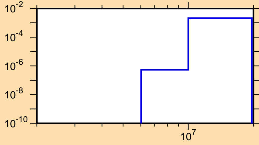
\sigma vs. E for ^{212}\text{Bi}(n,np)
