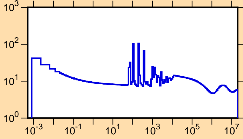
\sigma vs. E for ^{213}\text{Bi}(n,\text{tot.})
