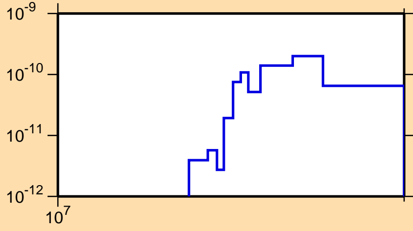
\sigma vs. E for ^{213}\text{Bi}(n,p\alpha)
