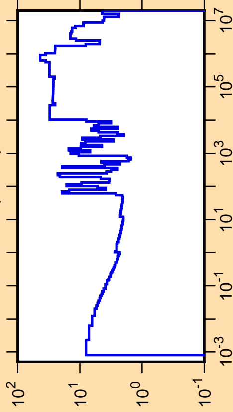
\Delta\sigma/\sigma vs. E for ^{213}\text{Bi}(n,\text{tot.})
