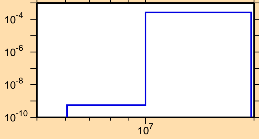
\sigma vs. E for ^{213}\text{Bi}(n,np)
