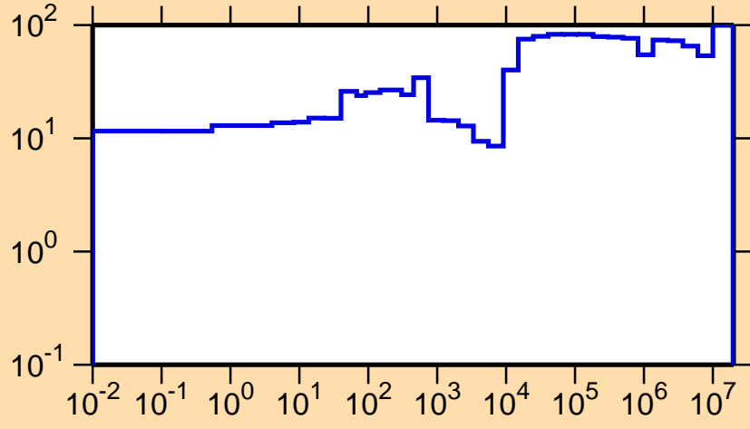
\Delta\sigma/\sigma vs. E for ^{213}\text{Bi}(n,\gamma)
