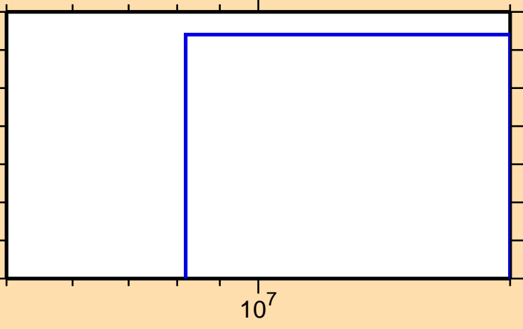
\sigma vs. E for ^{215}\text{Bi}(n,nt)
