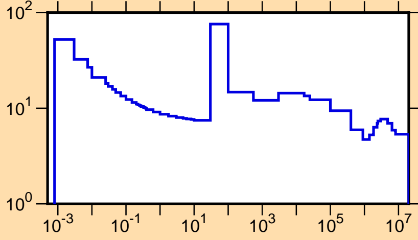
\sigma vs. E for ^{215}\text{Bi}(n,\text{tot.})
