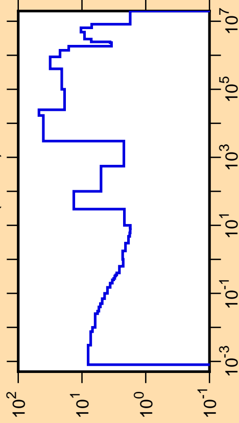
\Delta\sigma/\sigma vs. E for ^{215}\text{Bi}(n,\text{tot.})
