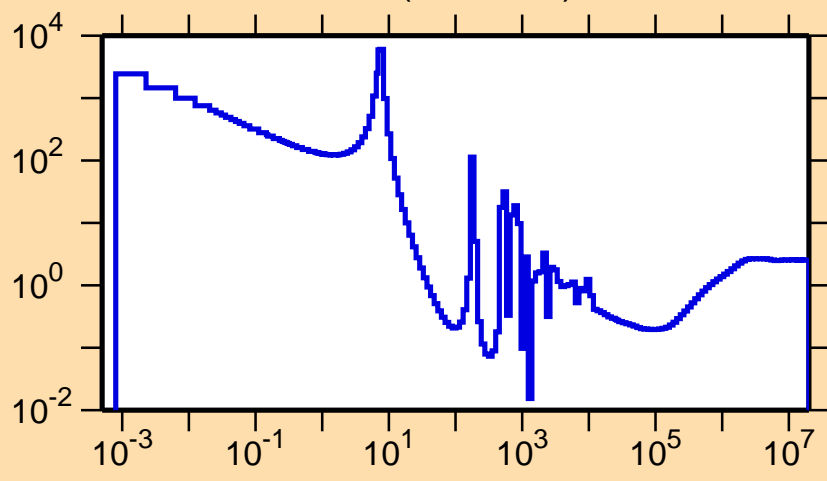
\sigma vs. E for ^{215}\text{Bi}(n,\text{nonel.})
