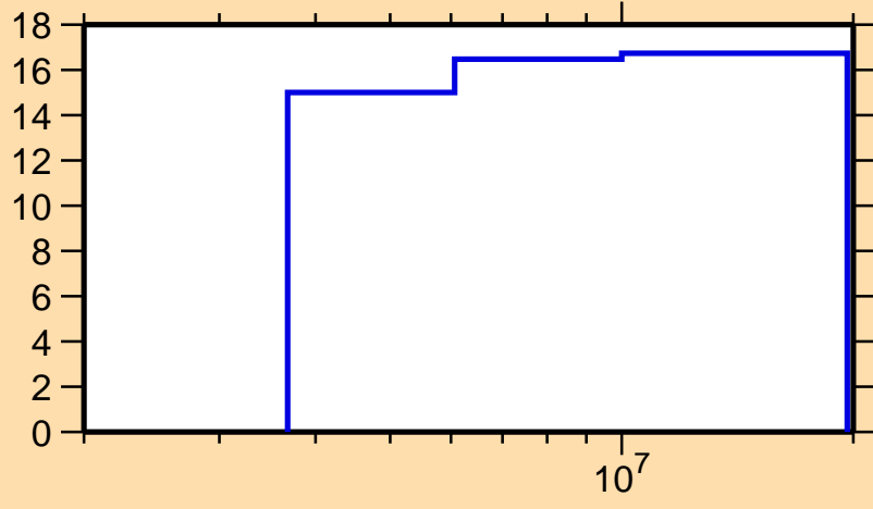
\Delta\sigma/\sigma vs. E for ^{215}\text{Bi}(n,\text{nonel.})
