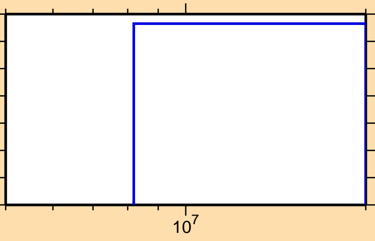
\sigma vs. E for ^{215}\text{Bi}(n,3n\alpha)
