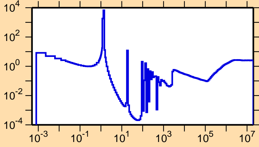
\sigma vs. E for ^{216}\text{Bi}(n,\text{nonel.})
