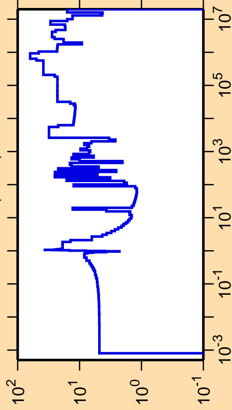
\Delta\sigma/\sigma vs. E for ^{216}\text{Bi}(n,\text{el.})
