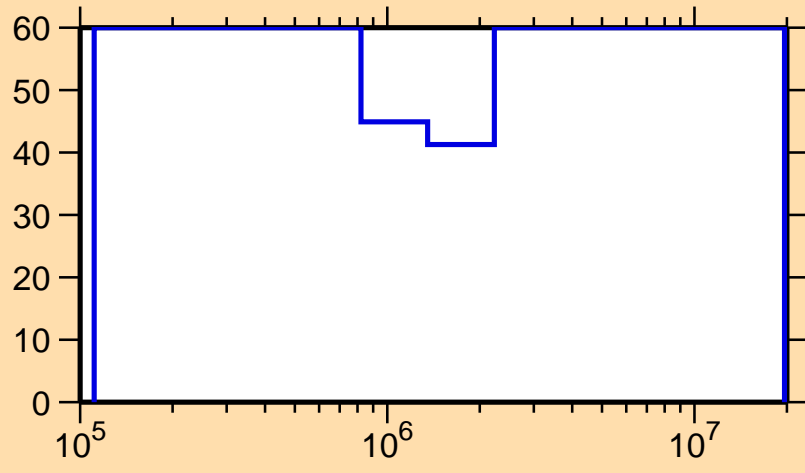
\Delta\sigma/\sigma vs. E for ^{216}\text{Bi}(n,n_1)
