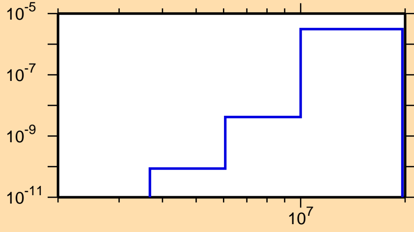
\sigma vs. E for ^{216}\text{Bi}(n,2n\alpha)
