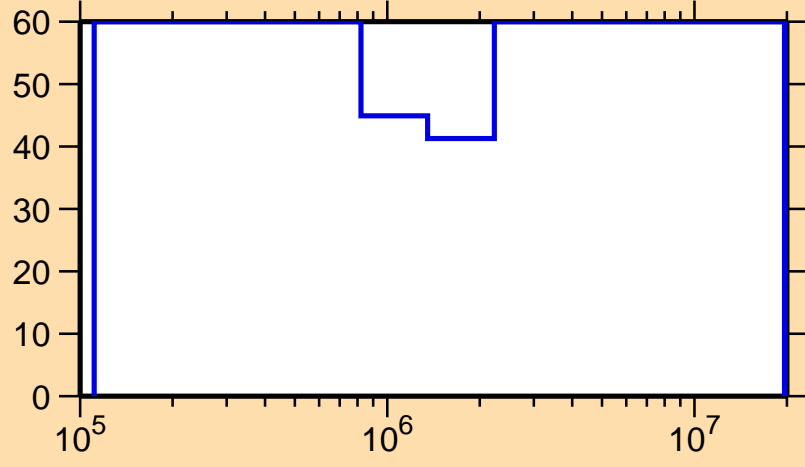
\Delta\sigma/\sigma vs. E for ^{216}\text{Bi}(n,n_1)
