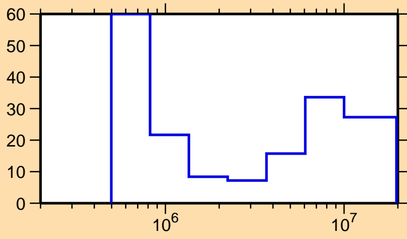
\Delta\sigma/\sigma vs. E for ^{216}\text{Bi}(n,n\text{cont.})
