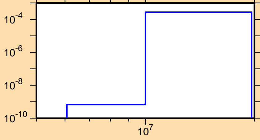
\sigma vs. E for ^{216}\text{Bi}(n,d)
