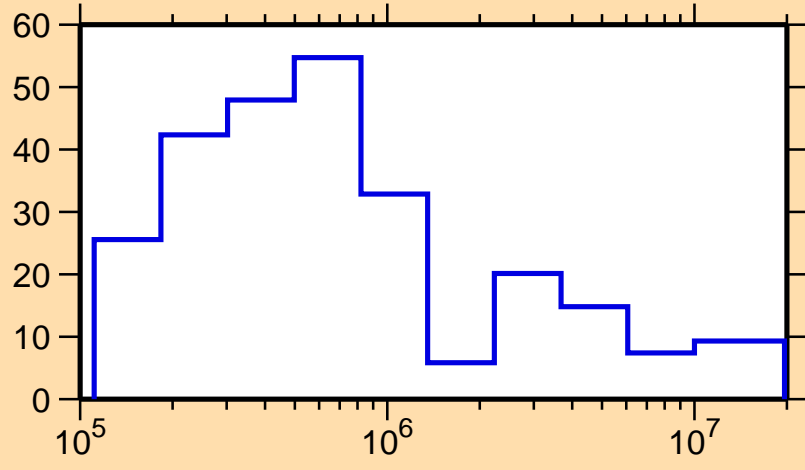
\Delta\sigma/\sigma vs. E for ^{216}\text{Bi}(n,\text{tot.})
