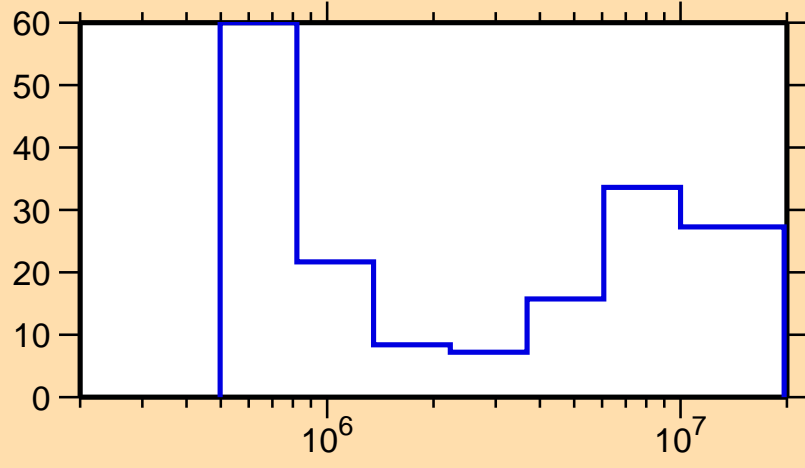
\Delta\sigma/\sigma vs. E for ^{216}\text{Bi}(n,n\text{cont.})
