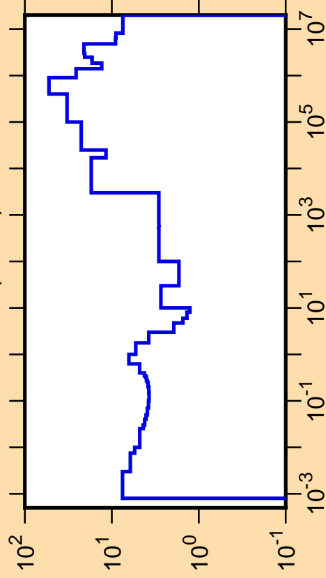
\Delta\sigma/\sigma vs. E for ^{216}\text{Bi}(n,\text{tot.})
