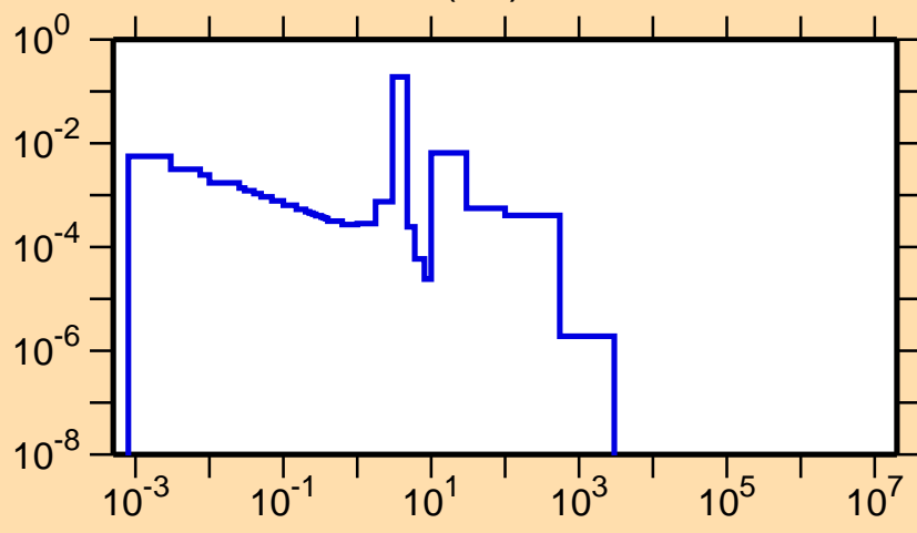
\sigma vs. E for ^{216}\text{Bi}(n,f)
