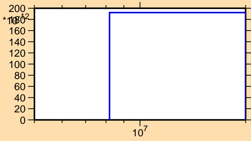
\sigma vs. E for ^{216}\text{Bi} (mt 11)
