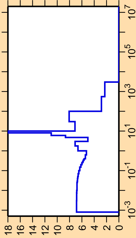
\Delta\sigma/\sigma vs. E for ^{216}\text{Bi}(n,f)
