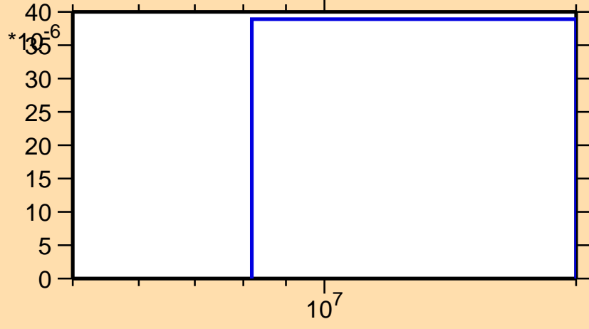
\sigma vs. E for ^{216}\text{Bi}(n,nt)
