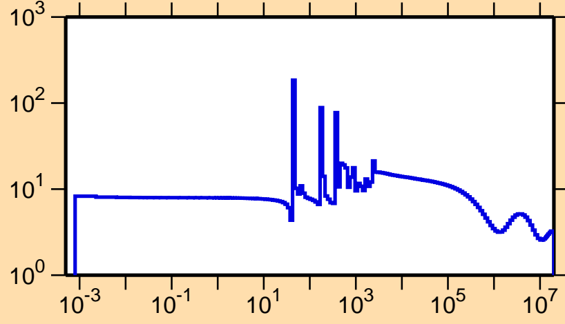
\sigma vs. E for ^{217}\text{Bi}(n,\text{el.})
