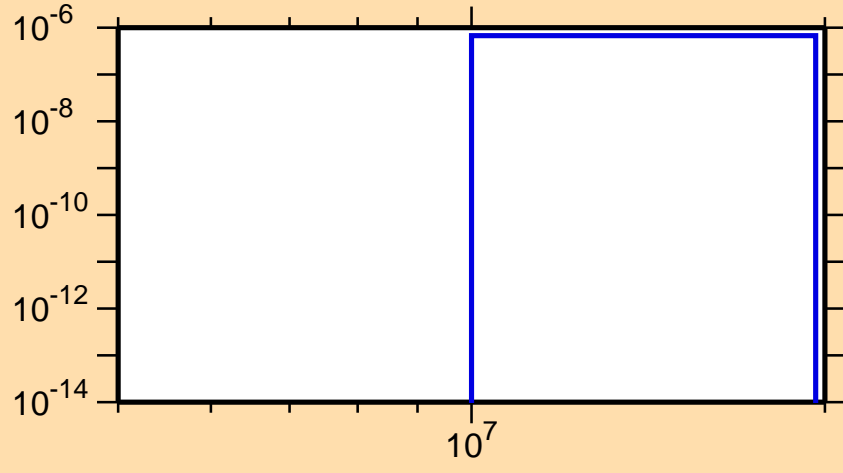
\sigma vs. E for ^{217}\text{Bi}(n,\text{nd})
