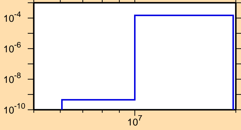
\sigma vs. E for ^{217}\text{Bi}(n,d)
