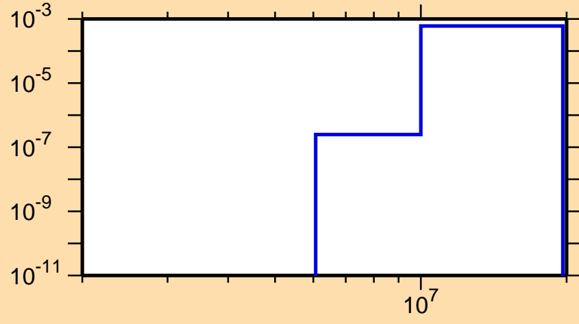
\sigma vs. E for ^{217}\text{Bi}(n,p)
