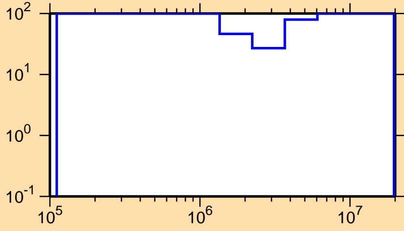
\Delta\sigma/\sigma vs. E for ^{217}\text{Bi}(n,n\text{cont.})
