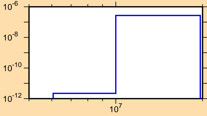
\sigma vs. E for ^{217}\text{Bi}(n,2n\alpha)
