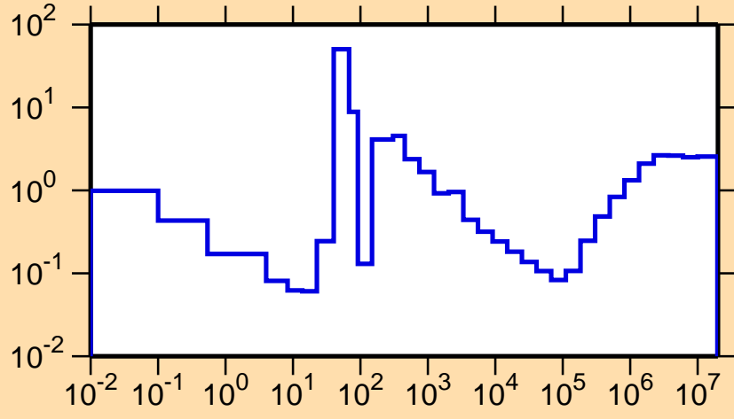
\sigma vs. E for ^{217}\text{Bi}(n,\text{nonel.})
