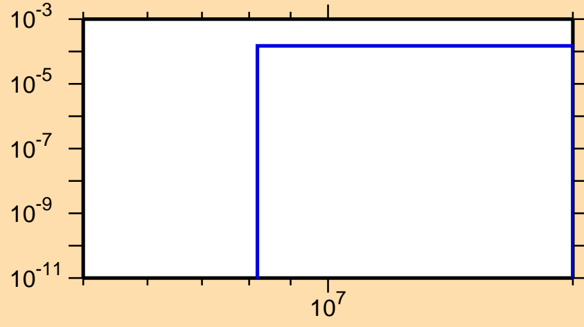
\sigma vs. E for ^{217}\text{Bi}(n,t)
