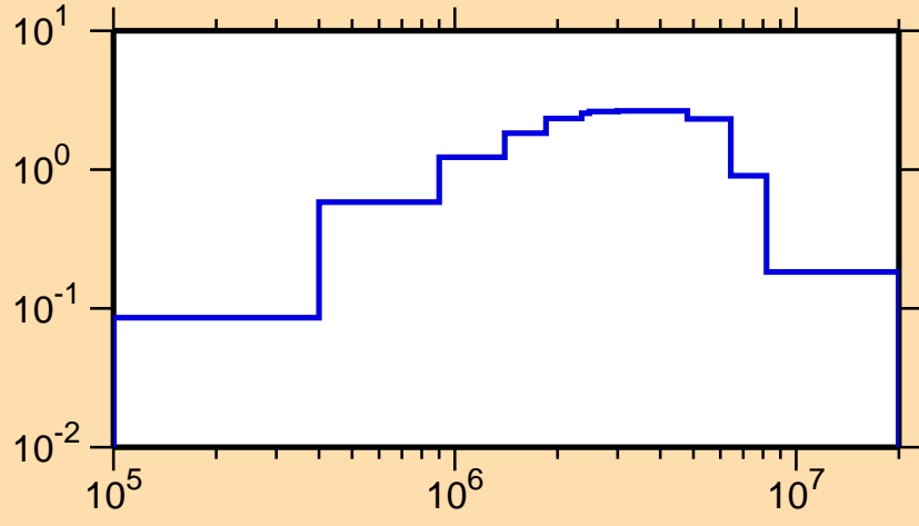
\sigma vs. E for ^{217}\text{Bi}(n,n\text{cont.})
