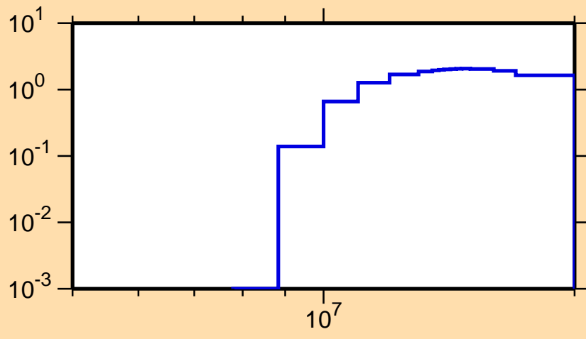
\sigma vs. E for ^{219}\text{Bi}(n,3n)
