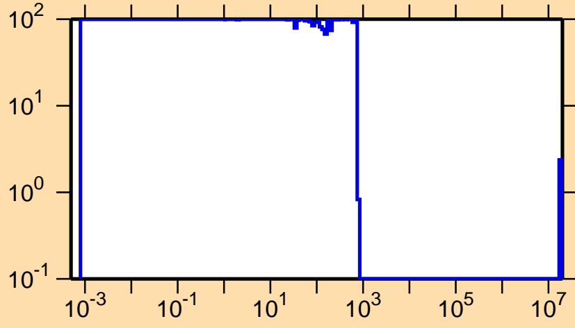
\Delta\sigma/\sigma vs. E for ^{219}\text{Bi}(n,f)
