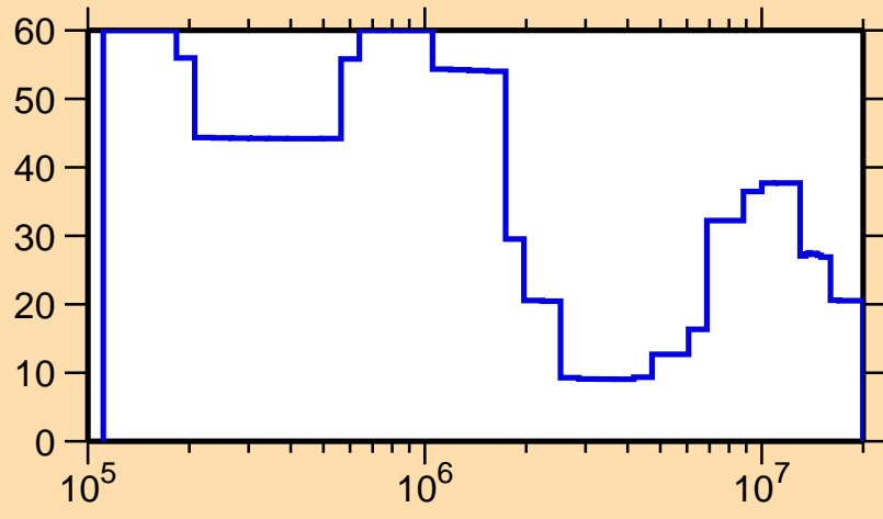
\Delta\sigma/\sigma vs. E for ^{219}\text{Bi}(n,\text{tot.})
