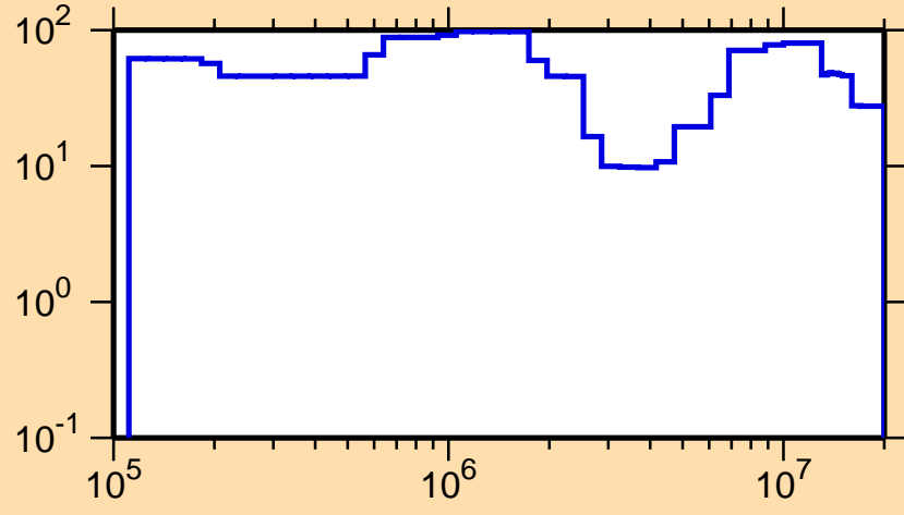
\Delta\sigma/\sigma vs. E for ^{219}\text{Bi}(n,\text{el.})
