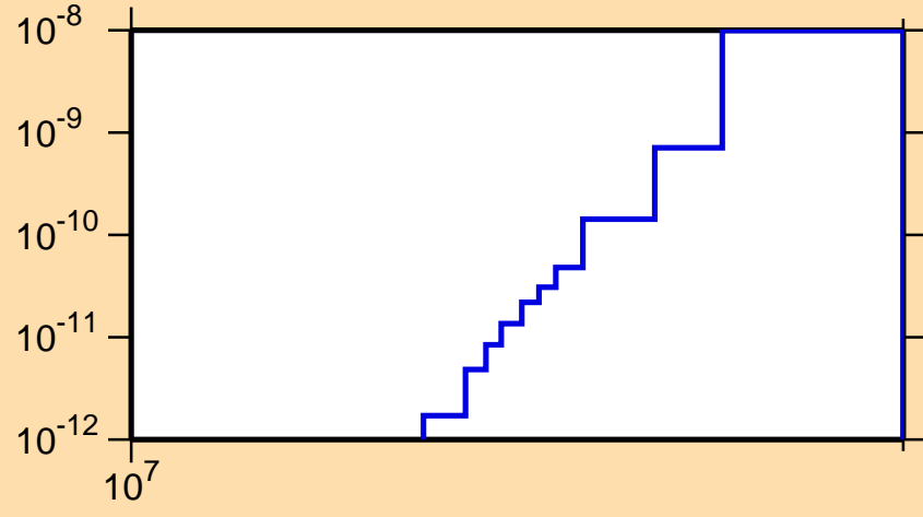
\sigma vs. E for ^{219}\text{Bi}(n,3n\alpha)
