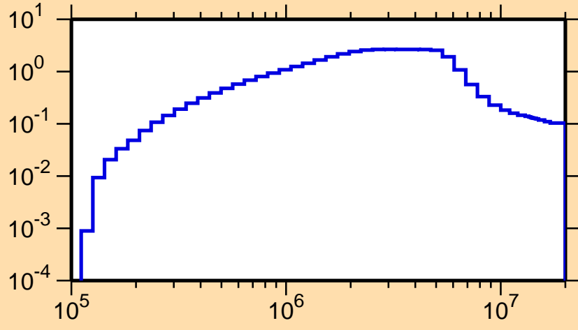
\sigma vs. E for ^{219}\text{Bi}(n,n\text{cont.})
