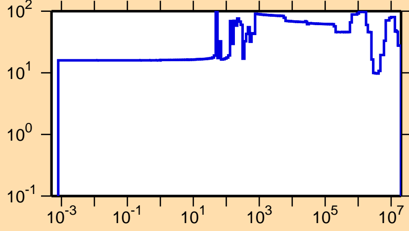
\Delta\sigma/\sigma vs. E for ^{219}\text{Bi}(n,el.)
