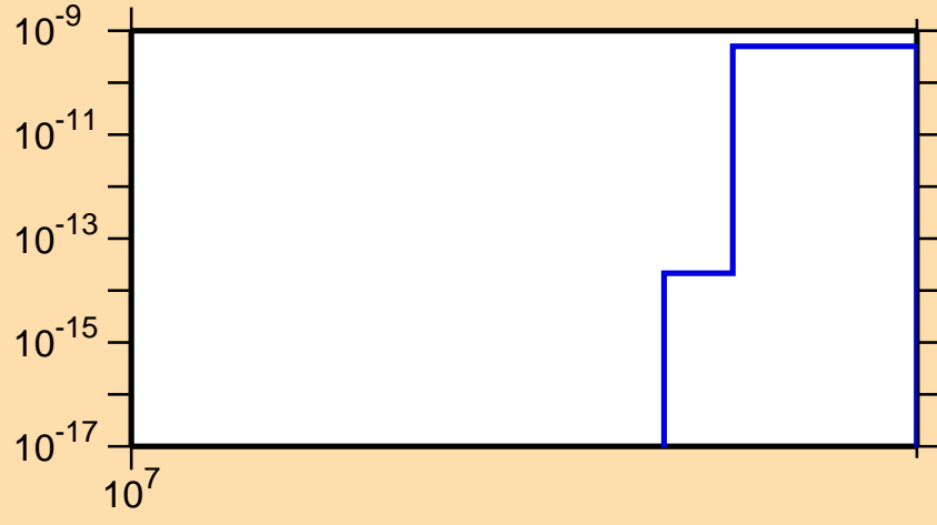
\sigma vs. E for ^{219}\text{Bi} (mt 42)
