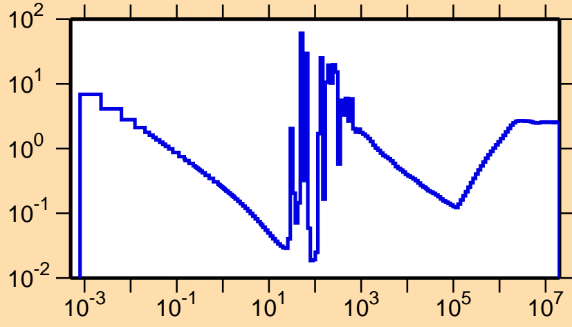
\sigma vs. E for ^{219}\text{Bi}(n,\text{nonel.})
