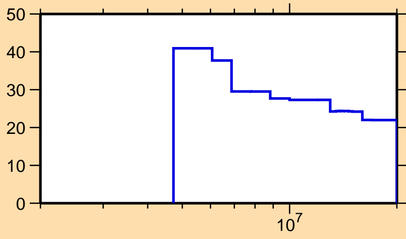
\Delta\sigma/\sigma vs. E for ^{219}\text{Bi}(n,\text{nonel.})
