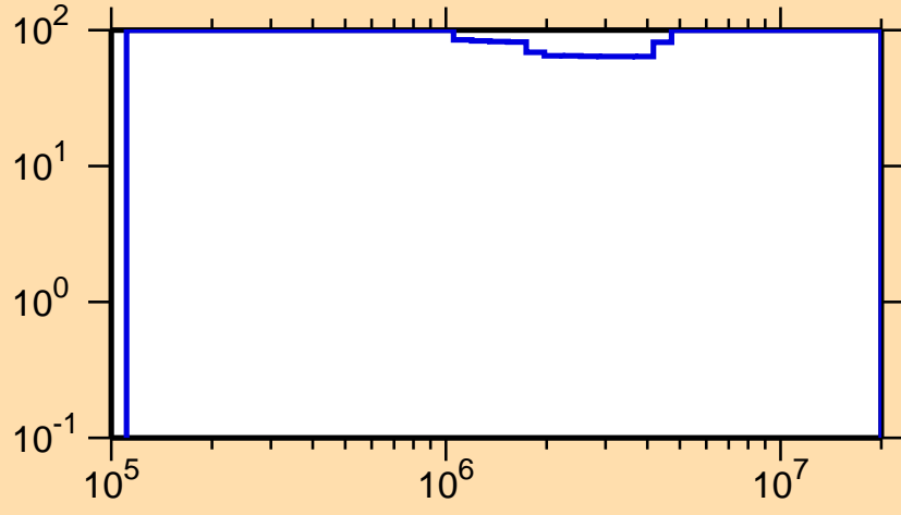
\Delta\sigma/\sigma vs. E for ^{219}\text{Bi}(n,n\text{cont.})
