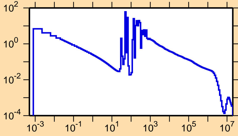
\sigma vs. E for ^{219}\text{Bi}(n,\gamma)
