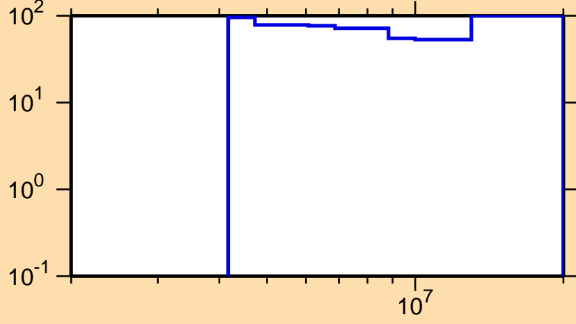
\Delta\sigma/\sigma vs. E for ^{219}\text{Bi}(n,\gamma)
