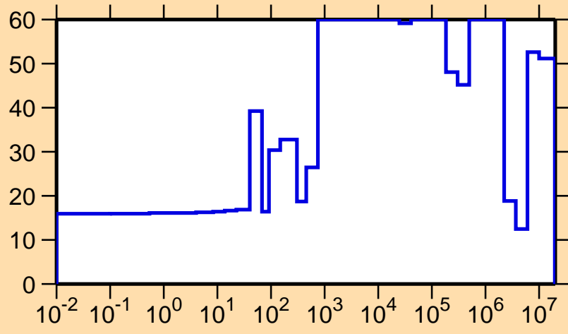
\Delta\sigma/\sigma vs. E for ^{219}\text{Bi}(n,el.)
