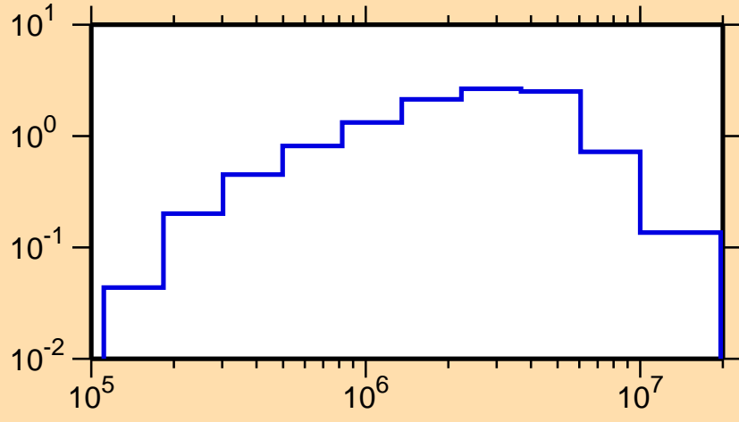
\sigma vs. E for ^{219}\text{Bi}(n,\text{inel.})
