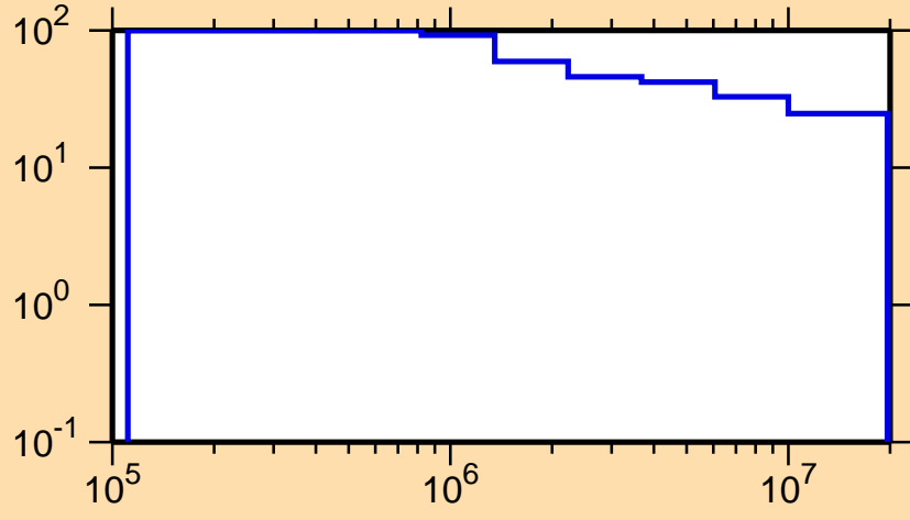
\Delta\sigma/\sigma vs. E for ^{219}\text{Bi}(n,n\text{onel.})
