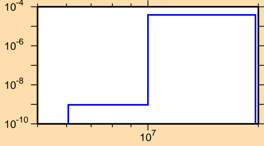
\sigma vs. E for ^{219}\text{Bi}(n,n\alpha)
