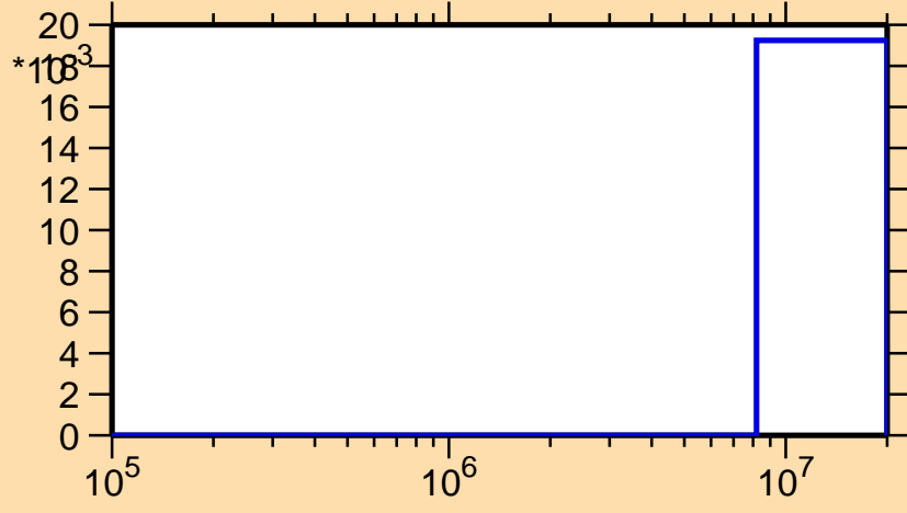
\Delta\sigma/\sigma vs. E for ^{219}\text{Bi}(n,\text{f})
