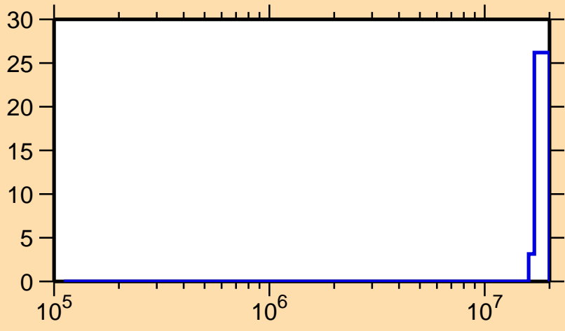
\Delta\sigma/\sigma vs. E for ^{220}\text{Bi}(n,f)
