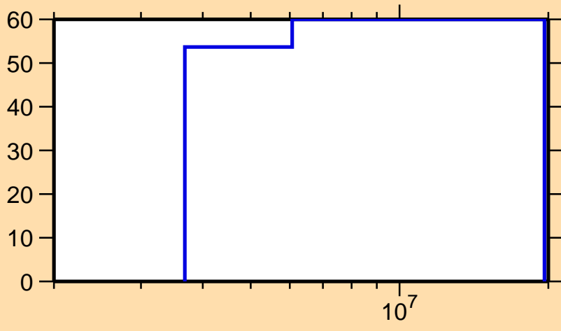
\Delta\sigma/\sigma vs. E for ^{220}\text{Bi}(n,p)
