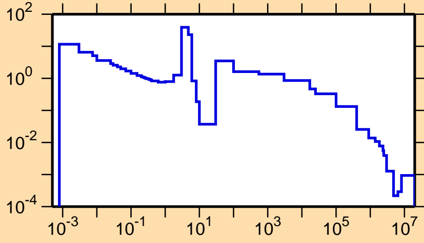
\sigma vs. E for ^{220}\text{Bi}(n,\gamma)
