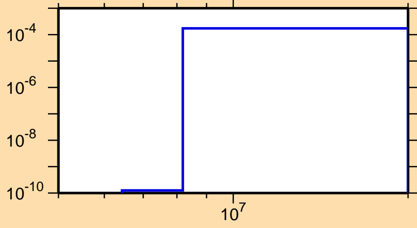
\sigma vs. E for ^{220}\text{Bi}(n,t)
