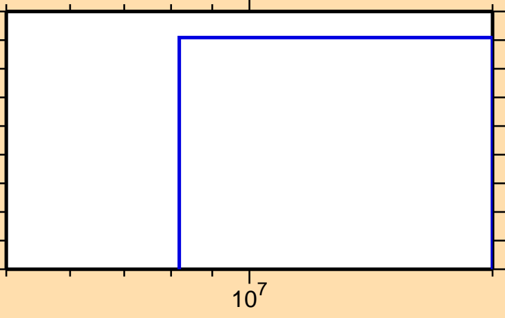
\sigma vs. E for ^{220}\text{Bi}(n,nt)
