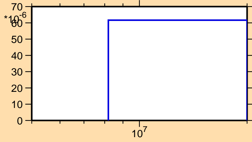
\sigma vs. E for ^{220}\text{Bi}(n,np)
