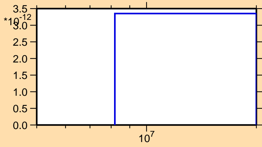
\sigma vs. E for ^{220}\text{Bi} (mt 42)
