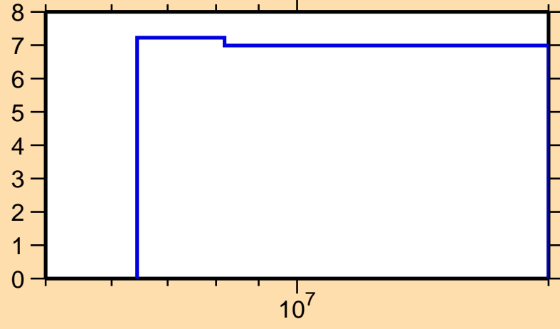
\Delta\sigma/\sigma vs. E for ^{221}\text{Bi}(n,\text{nonel.})
