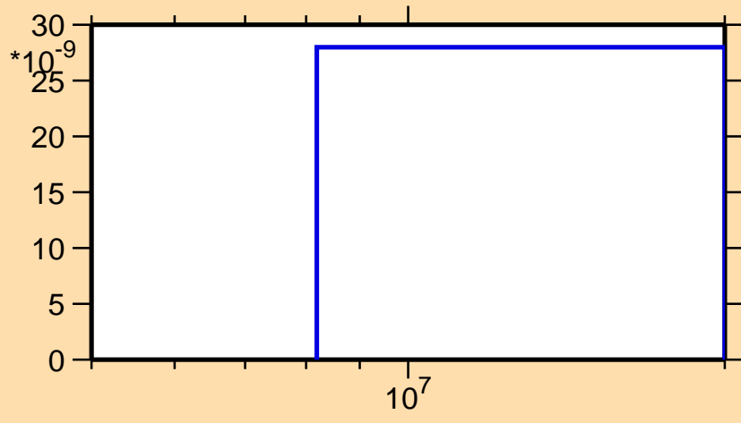
\sigma vs. E for ^{221}\text{Bi}(n,2n\alpha)
