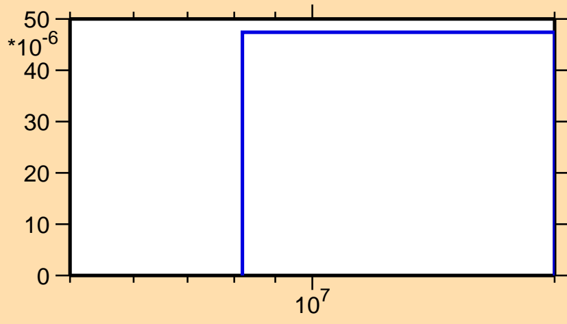
\sigma vs. E for ^{221}\text{Bi}(n,d)
