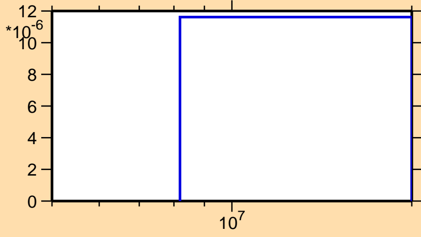
\sigma vs. E for ^{221}\text{Bi}(n,nt)
