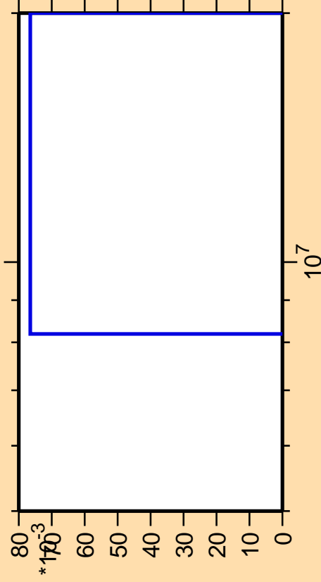
\Delta\sigma/\sigma vs. E for ^{221}\text{Bi} (mt 42)
