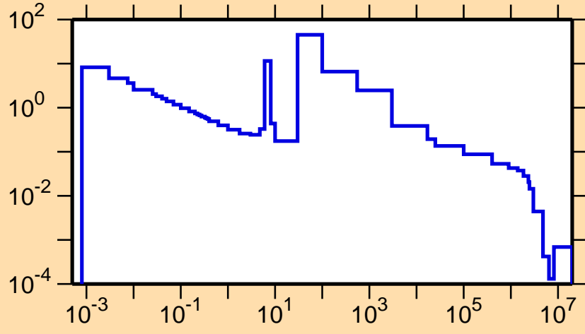
\sigma vs. E for ^{221}\text{Bi}(n,\gamma)
