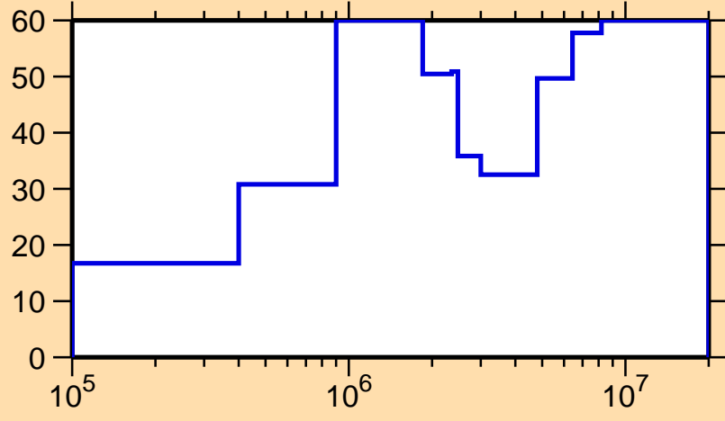
\Delta\sigma/\sigma vs. E for ^{221}\text{Bi}(n, tot.)
