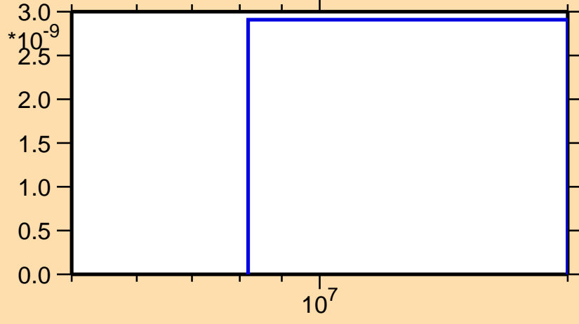
\sigma vs. E for ^{221}\text{Bi}(n,2np)
