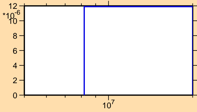
\sigma vs. E for ^{221}\text{Bi}(n,np)
