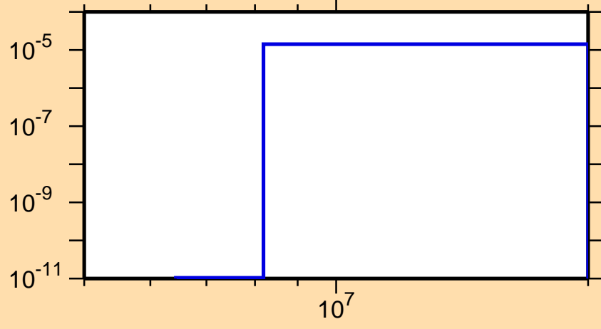
\sigma vs. E for ^{221}\text{Bi}(n,n\alpha)
