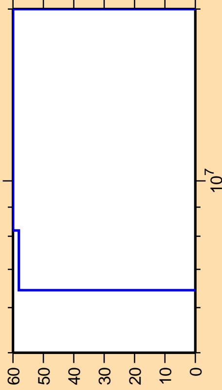
\Delta\sigma/\sigma vs. E for ^{221}\text{Bi}(n,n\alpha)
