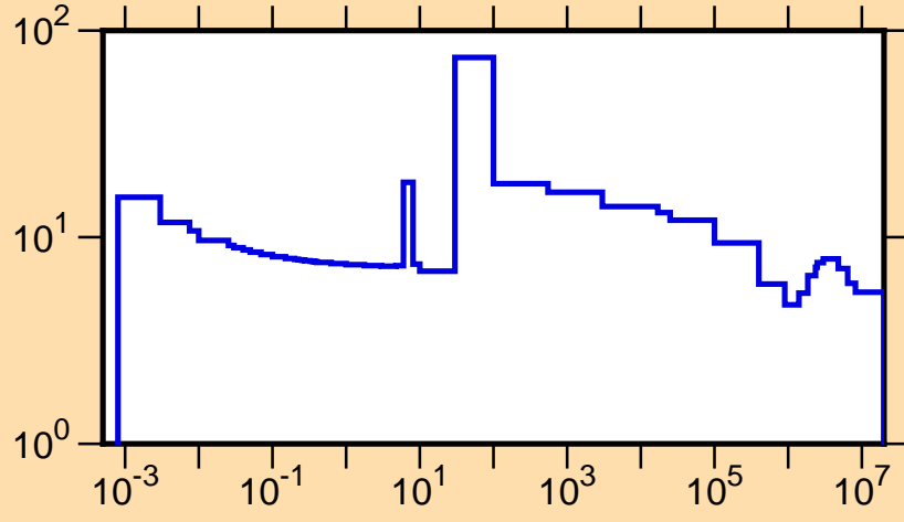
\sigma vs. E for ^{221}\text{Bi}(n,\text{tot.})
