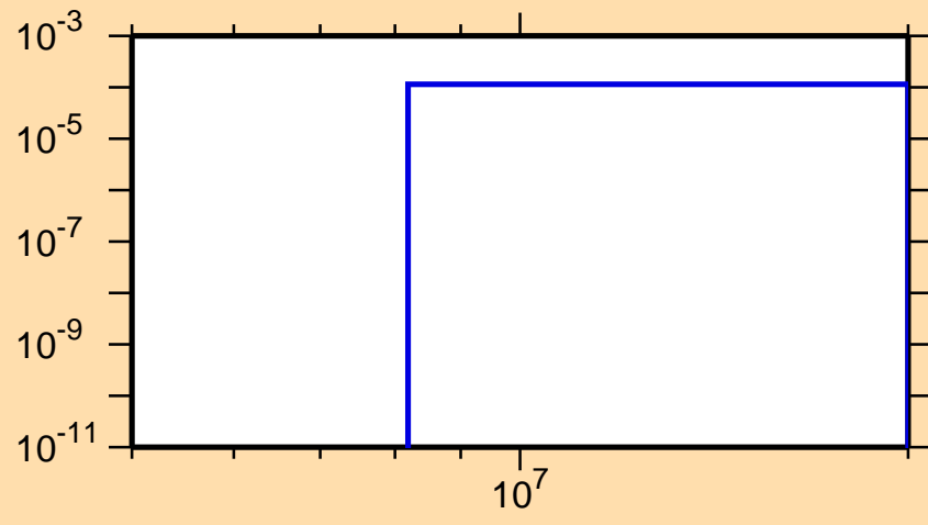
\sigma vs. E for ^{221}\text{Bi}(n,p)
