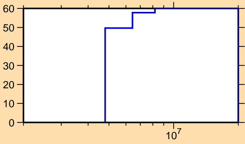
\Delta\sigma/\sigma vs. E for ^{221}\text{Bi}(n,\text{tot.})
