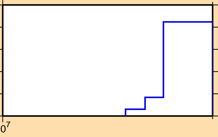
\sigma vs. E for ^{223}\text{Bi} (mt 42)
