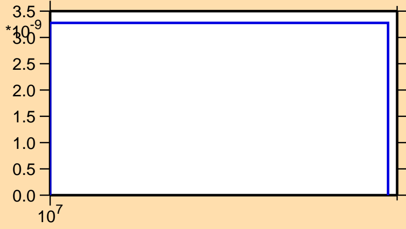
\sigma vs. E for ^{223}\text{Bi}(n,2n\alpha)
