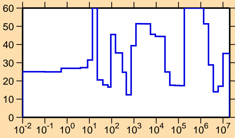
\Delta\sigma/\sigma vs. E for ^{223}\text{Bi}(n,el.)
