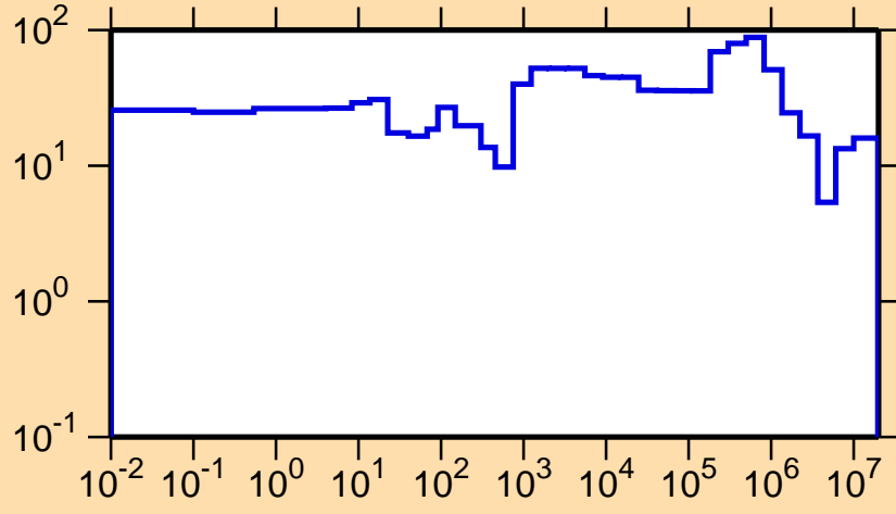
\Delta\sigma/\sigma vs. E for ^{223}\text{Bi}(n,tot.)
