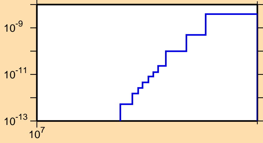
\sigma vs. E for ^{234}\text{Bk}(n,2np)
