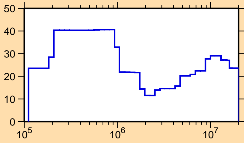
\Delta\sigma/\sigma vs. E for ^{234}\text{Bk}(n,\text{el.})
