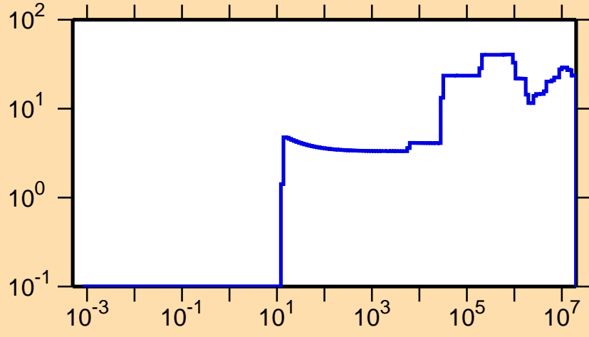
\Delta\sigma/\sigma vs. E for ^{234}\text{Bk}(n,el.)
