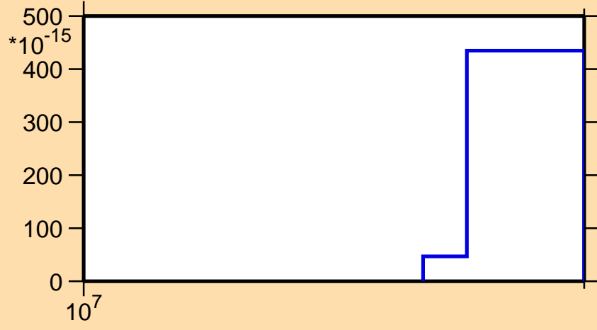
\sigma vs. E for ^{234}\text{Bk}(n,pd)
