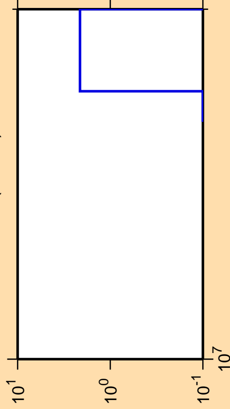
\Delta\sigma/\sigma vs. E for ^{234}\text{Bk}(n,3n\alpha)
