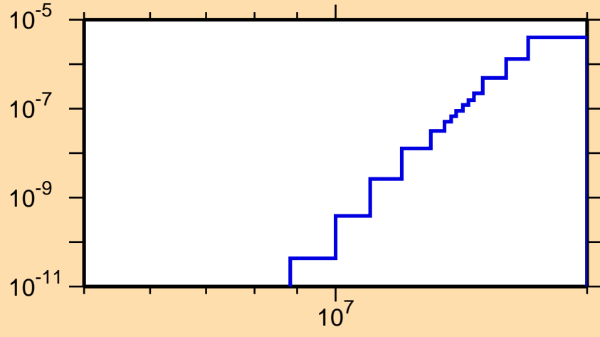
\sigma vs. E for ^{234}\text{Bk}(n,\text{He}3)
