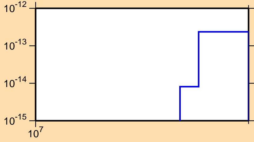
\sigma vs. E for ^{234}\text{Bk}(n,3n\alpha)
