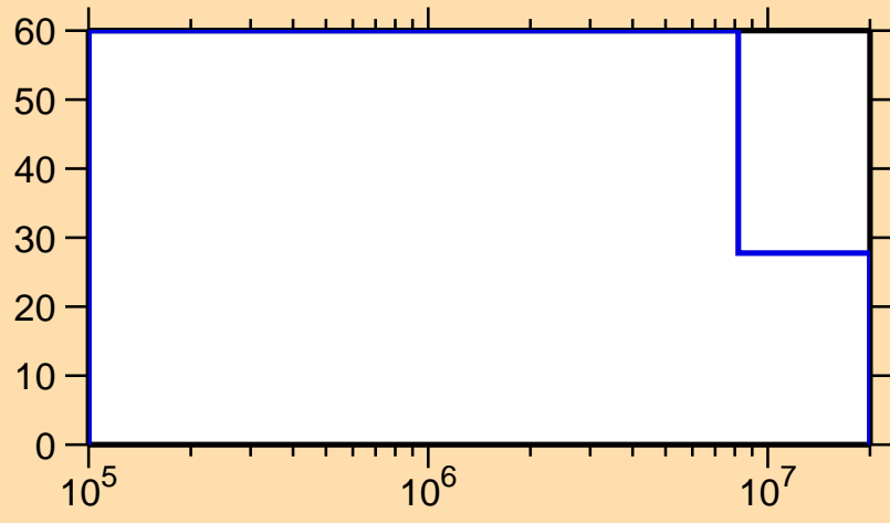
\Delta\sigma/\sigma vs. E for ^{234}\text{Bk}(n,n_1)
