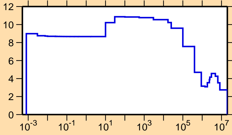
\sigma vs. E for ^{234}\text{Bk}(n,\text{el.})
