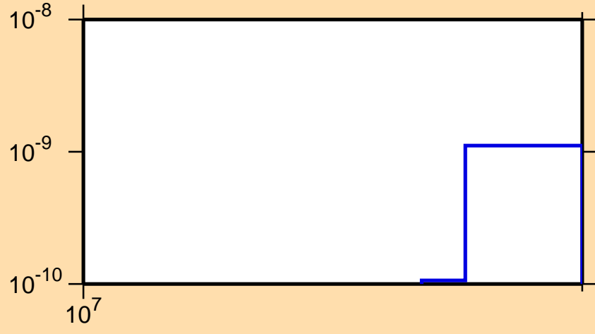
\sigma vs. E for ^{235}\text{Bk}(n,nd)
