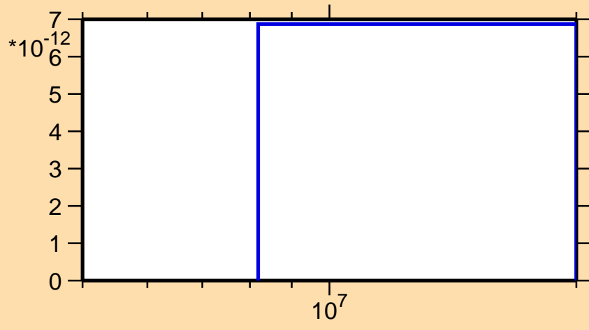
\sigma vs. E for ^{235}\text{Bk}(n,2np)
