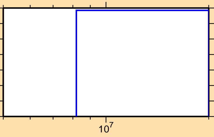
\sigma vs. E for ^{235}\text{Bk}(n,2n\alpha)
