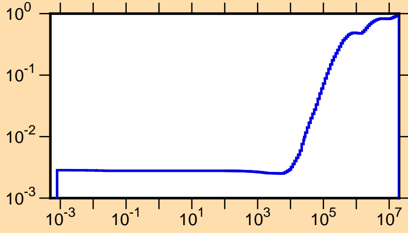
\mu vs. E for ^{236}\text{Bk}(\text{mt251})
