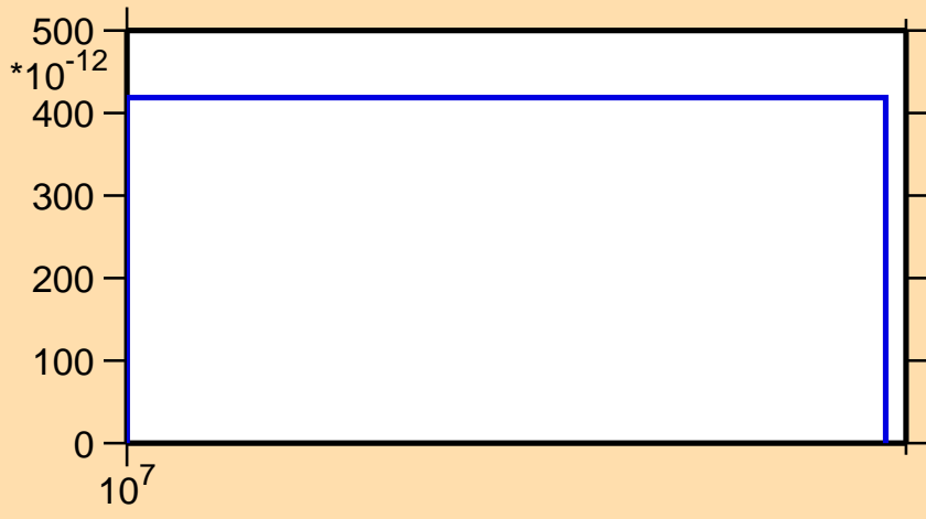
\sigma vs. E for ^{236}\text{Bk}(n,nd)
