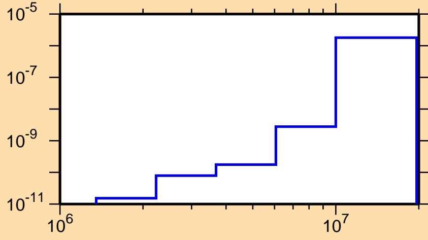
\sigma vs. E for ^{236}\text{Bk}(n,n\alpha)
