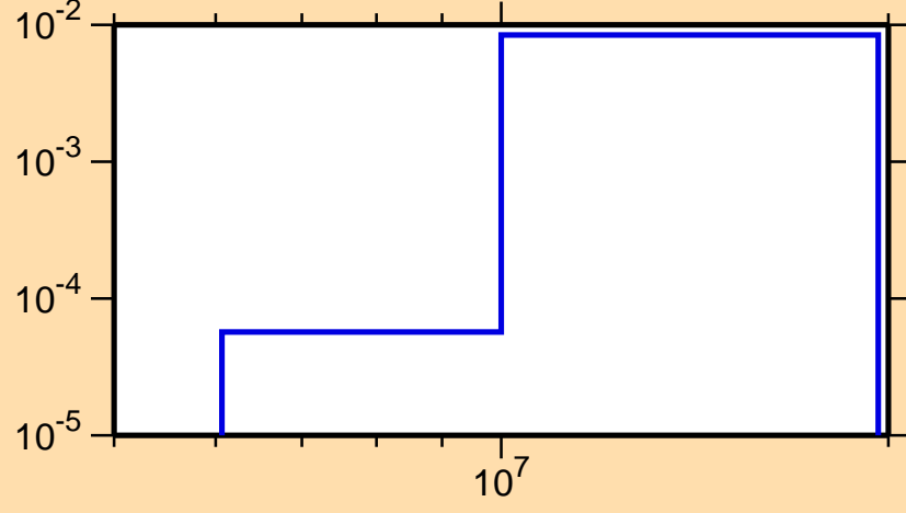
\sigma vs. E for ^{236}\text{Bk}(n,2n)
