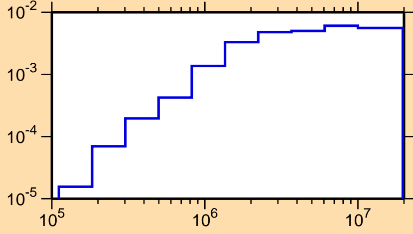
\sigma vs. E for ^{236}\text{Bk}(n,n\text{cont.})
