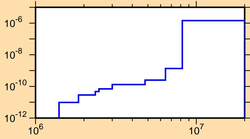
\sigma vs. E for ^{236}\text{Bk}(n,n\alpha)
