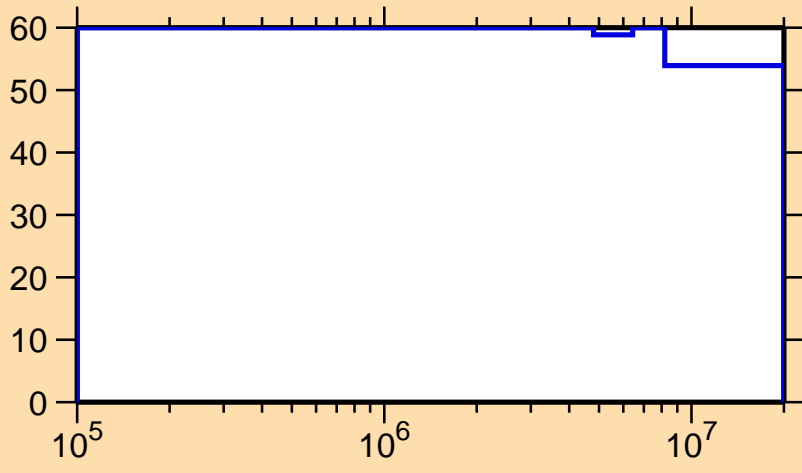
\Delta\sigma/\sigma vs. E for ^{236}\text{Bk}(n,n_1)
