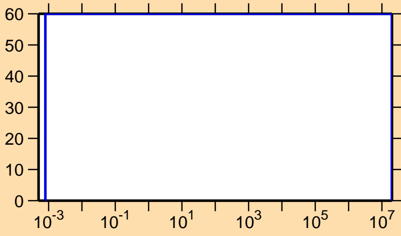
\Delta\sigma/\sigma vs. E for ^{236}\text{Bk}(n,\gamma)
