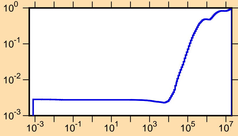
\mu vs. E for ^{237}\text{Bk}(\text{mt251})
