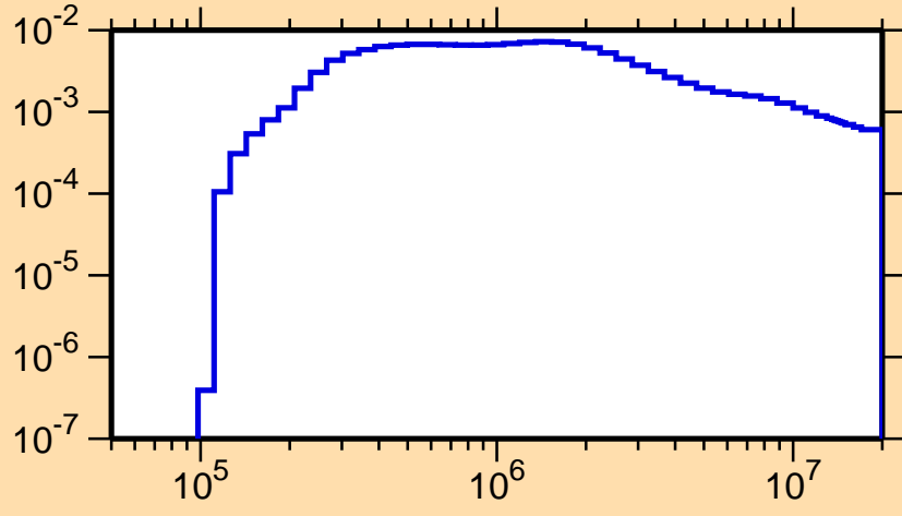
\sigma vs. E for ^{237}\text{Bk}(n,n_1)
