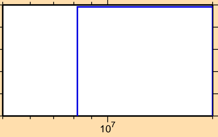
\sigma vs. E for ^{237}\text{Bk}(n,\text{He3})
