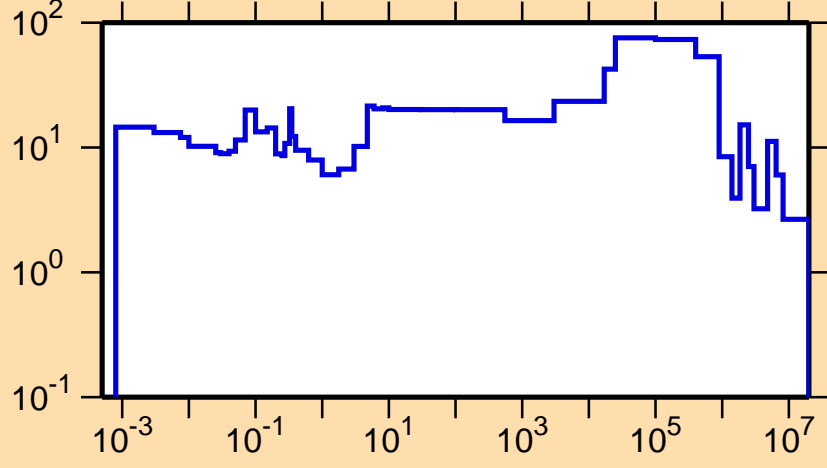
\Delta\sigma/\sigma vs. E for ^{237}\text{Bk}(n,tot.)
