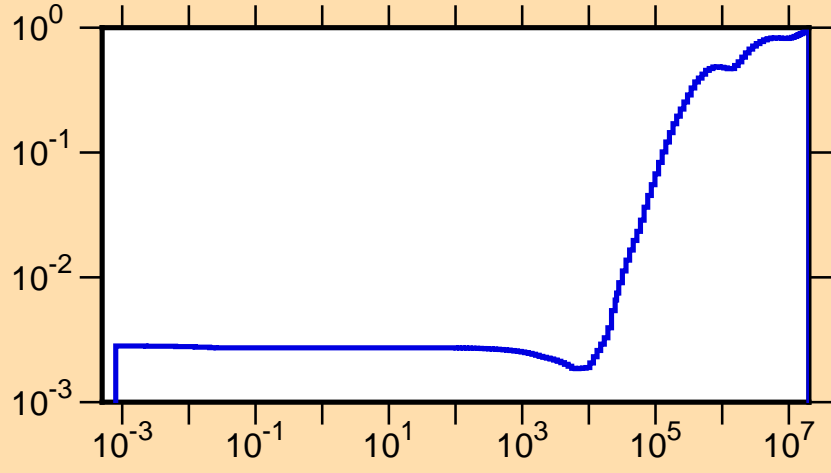
\mu vs. E for ^{238}\text{Bk}(\text{mt251})
