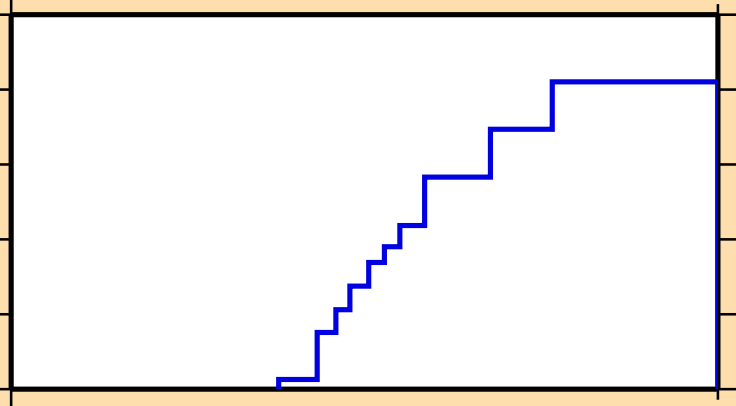
\sigma vs. E for ^{238}\text{Bk}(n,2np)
