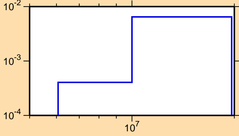
\sigma vs. E for ^{238}\text{Bk}(n,2n)
