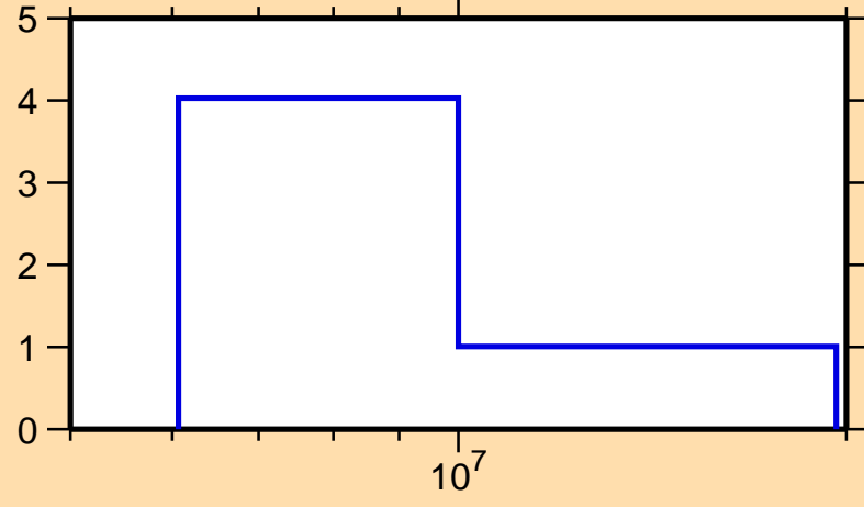
\Delta\sigma/\sigma vs. E for ^{238}\text{Bk}(n,\text{tot.})
