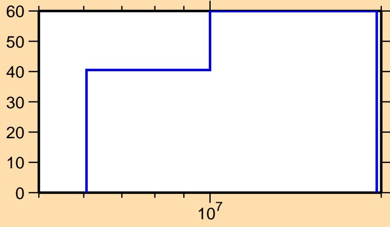
\Delta\sigma/\sigma vs. E for ^{238}\text{Bk}(n,2n)
