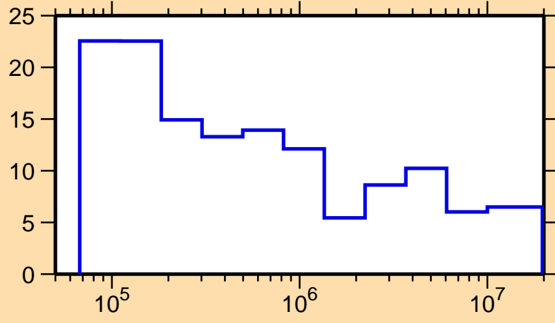
\Delta\sigma/\sigma vs. E for ^{238}\text{Bk}(n,\text{nonel.})
