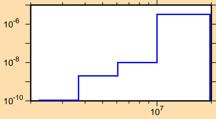
\sigma vs. E for ^{238}\text{Bk}(n,n\alpha)
