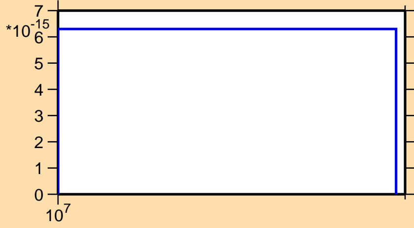
\sigma vs. E for ^{238}\text{Bk}(n,3n\alpha)
