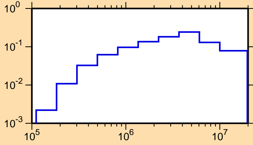
\sigma vs. E for ^{238}\text{Bk}(n,\text{inel.})
