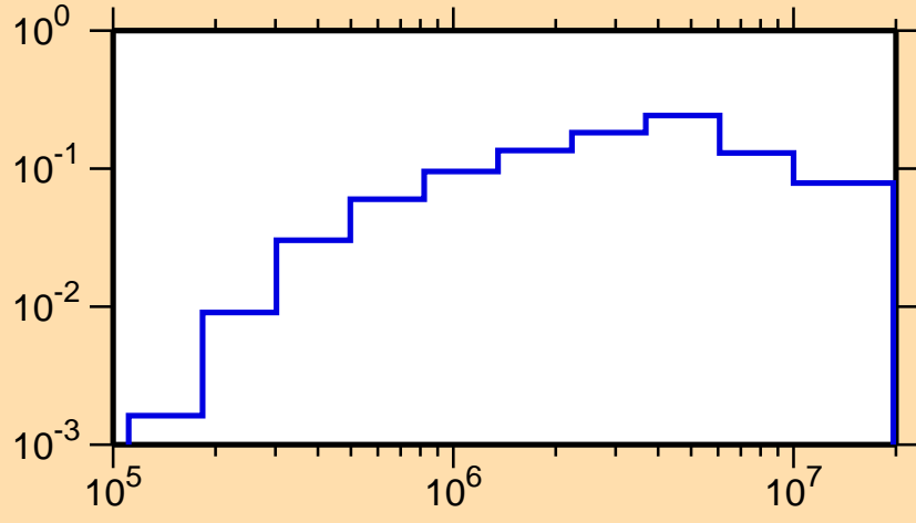
\sigma vs. E for ^{238}\text{Bk}(n,n\text{cont.})
