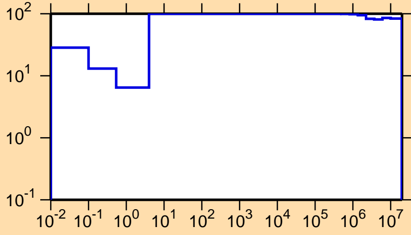
\Delta\sigma/\sigma vs. E for ^{238}\text{Bk}(n,\gamma)
