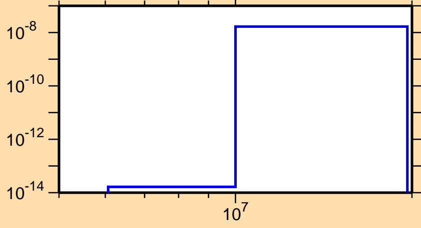
\sigma vs. E for ^{238}\text{Bk}(n,\text{He3})
