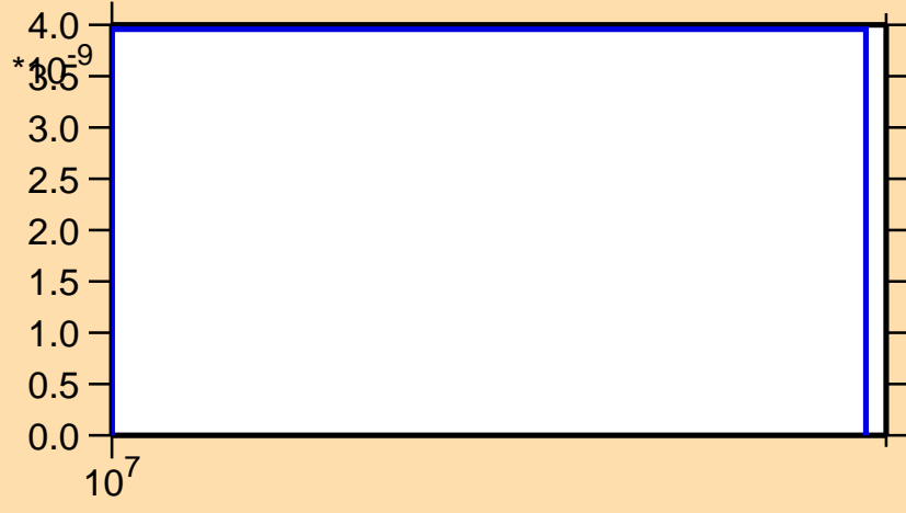
\sigma vs. E for ^{238}\text{Bk}(n,2np)
