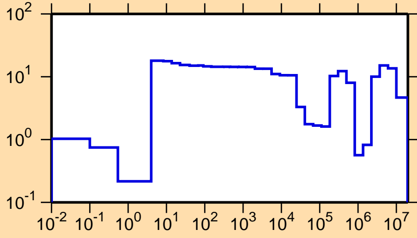
\Delta\sigma/\sigma vs. E for ^{238}\text{Bk}(n,\text{el.})
