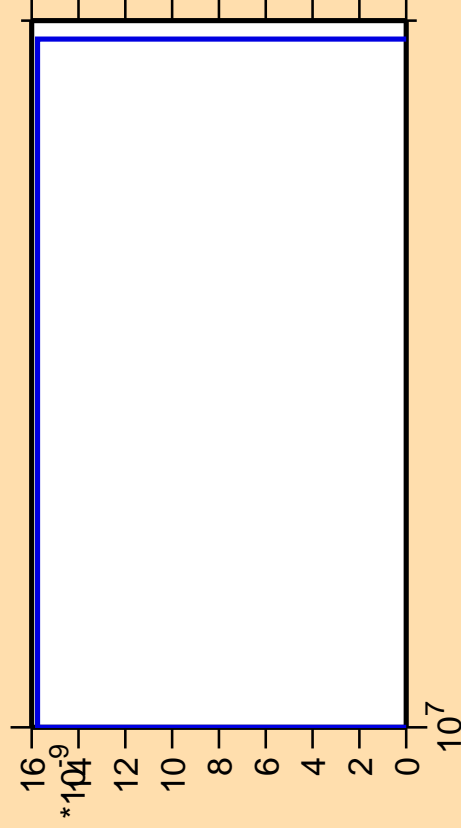
\Delta\sigma/\sigma vs. E for ^{238}\text{Bk}(n,3n\alpha)
