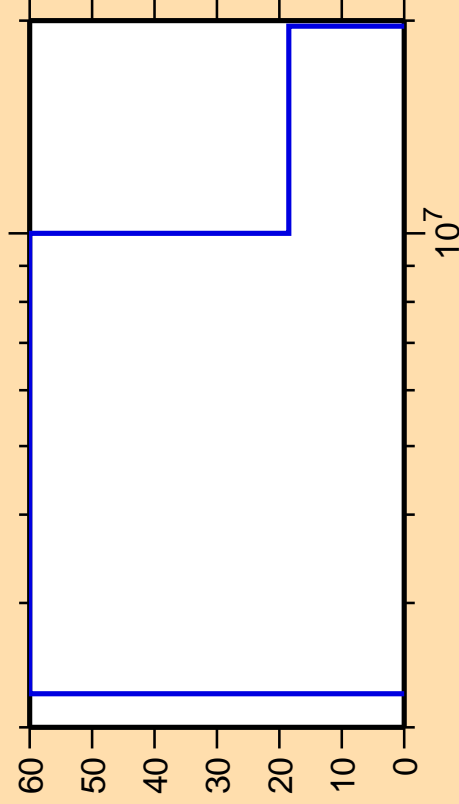
\Delta\sigma/\sigma vs. E for ^{238}\text{Bk}(n,n\alpha)
