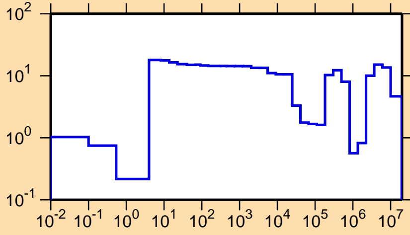
\Delta\sigma/\sigma vs. E for ^{238}\text{Bk}(n,el.)
