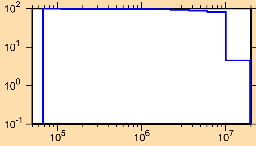
\Delta\sigma/\sigma vs. E for ^{238}\text{Bk}(n,n_1)
