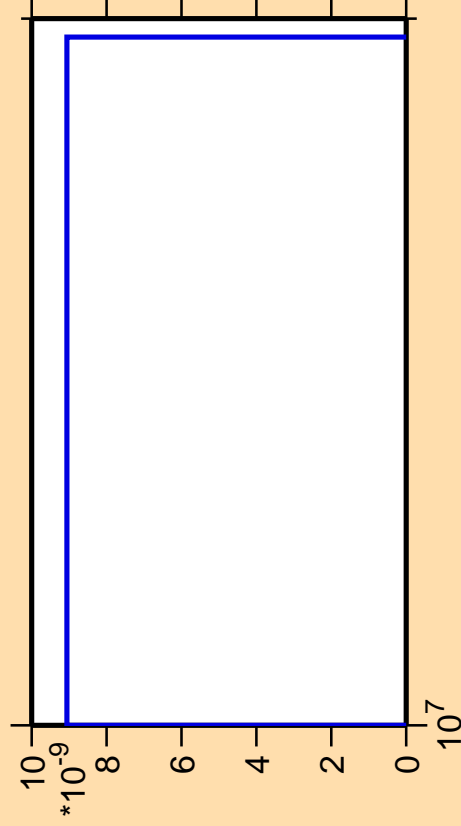
\Delta\sigma/\sigma vs. E for ^{238}\text{Bk} (mt 34)
