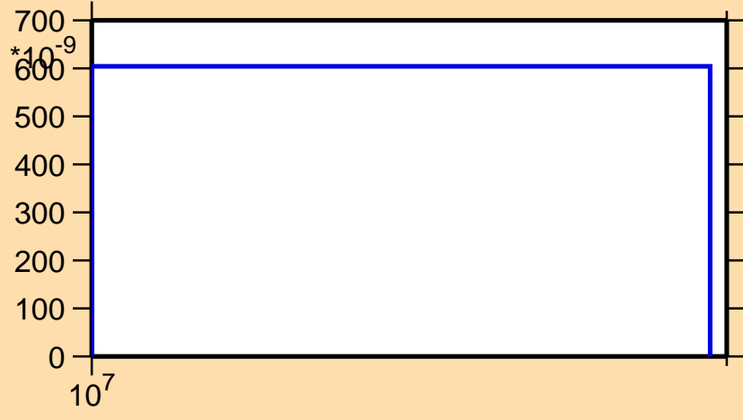
\sigma vs. E for ^{238}\text{Bk}(n,3n)
