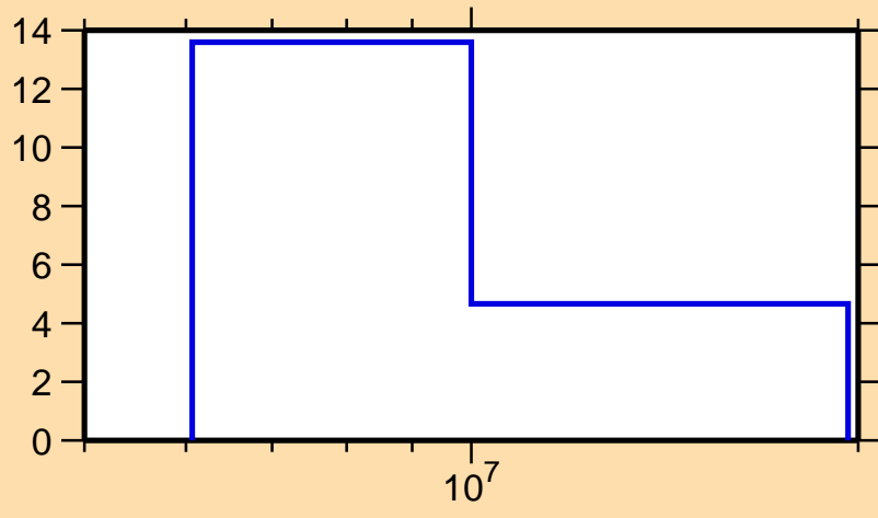
\Delta\sigma/\sigma vs. E for ^{238}\text{Bk}(n,\text{el.})
