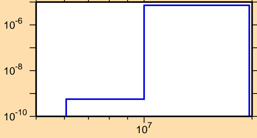
\sigma vs. E for ^{238}\text{Bk}(n,t)
