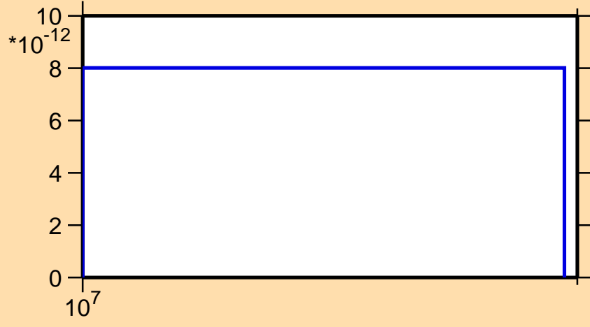
\sigma vs. E for ^{238}\text{Bk}(n,nt)
