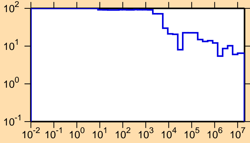
\Delta\sigma/\sigma vs. E for ^{238}\text{Bk}(n,\text{nonel.})
