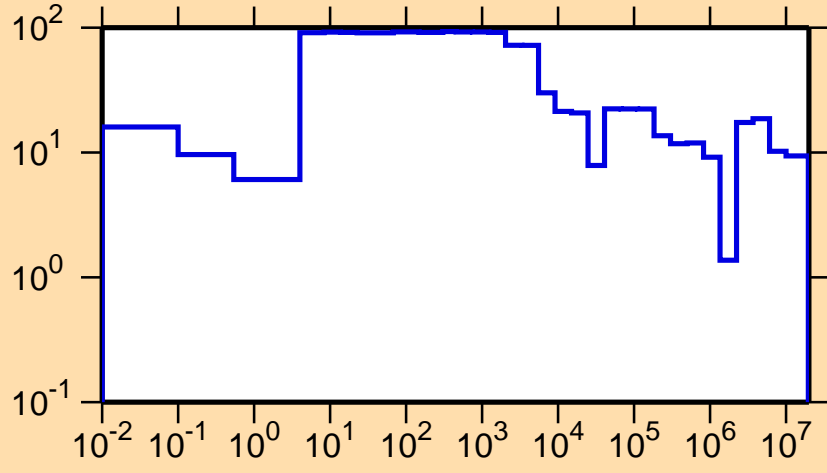
\Delta\sigma/\sigma vs. E for ^{238}\text{Bk}(n,f)
