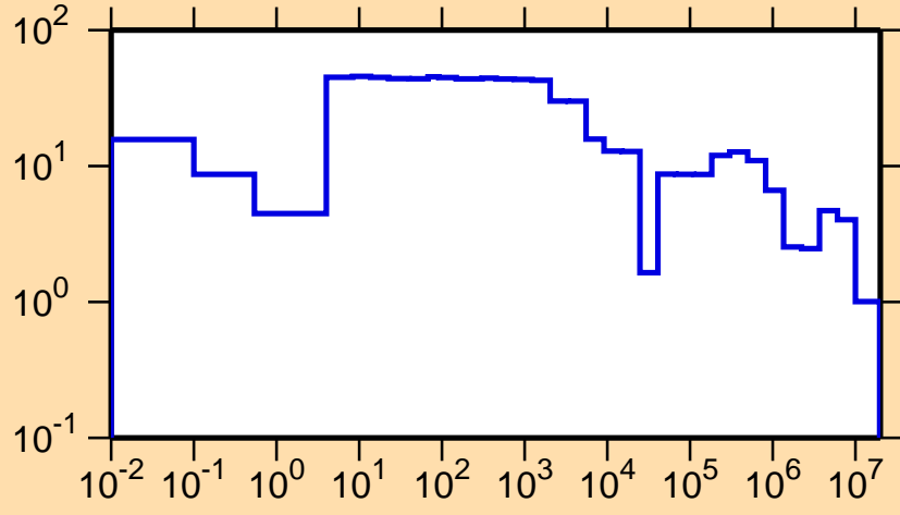
\Delta\sigma/\sigma vs. E for ^{238}\text{Bk}(n,\text{tot.})
