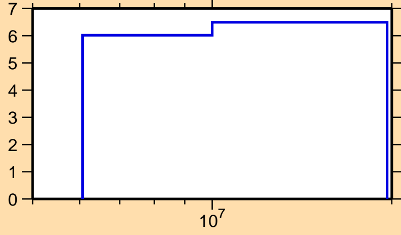
\Delta\sigma/\sigma vs. E for ^{238}\text{Bk}(n,\text{nonel.})
