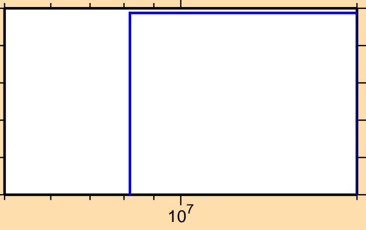
\sigma vs. E for ^{238}\text{Bk}(n,nd)
