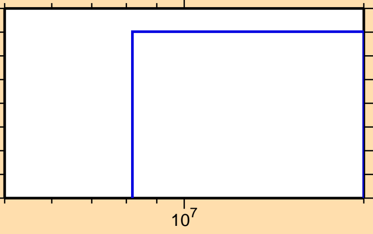
\sigma vs. E for ^{238}\text{Bk}(n,nt)
