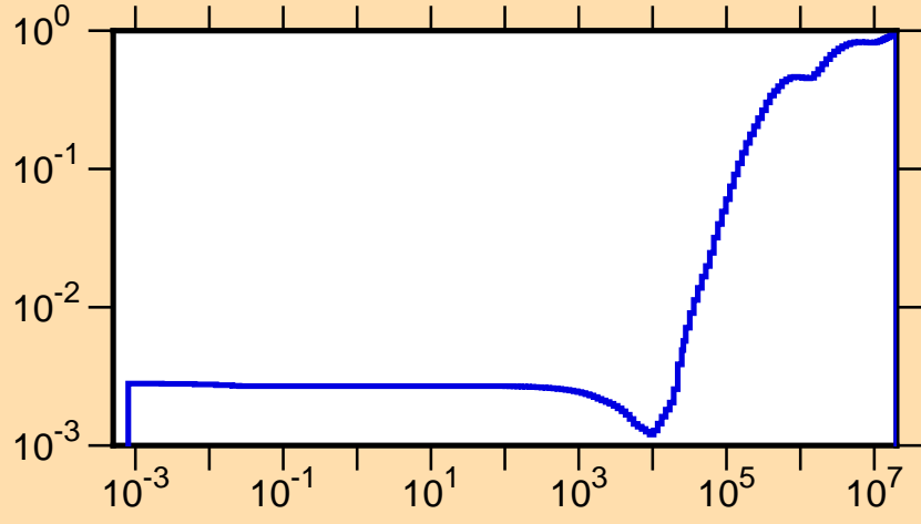
\mu vs. E for ^{239}\text{Bk}(\text{mt251})
