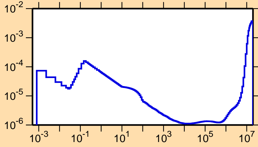
\sigma vs. E for ^{239}\text{Bk}(n,\alpha)
