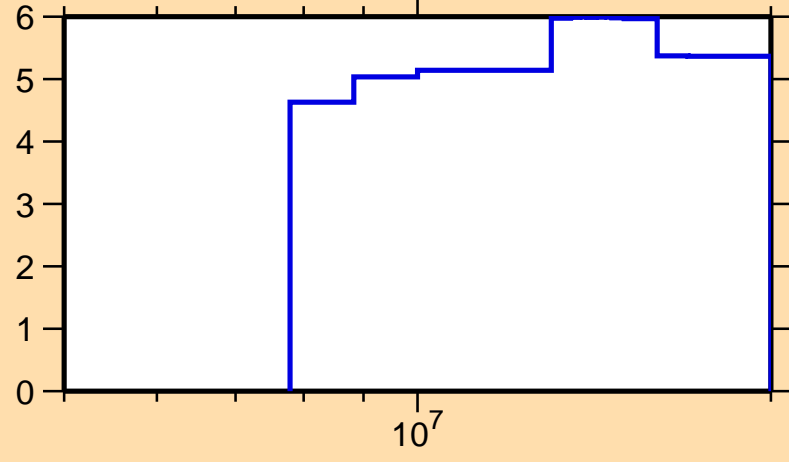
\Delta\sigma/\sigma vs. E for ^{239}\text{Bk}(n,\text{nonel.})
