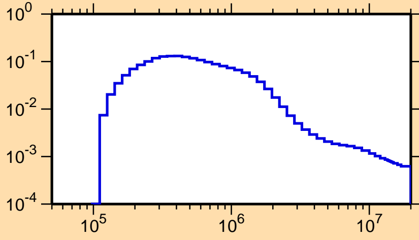
\sigma vs. E for ^{239}\text{Bk}(n,n_1)
