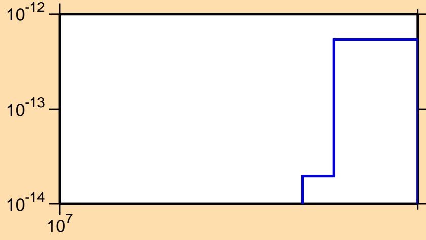
\sigma vs. E for ^{239}\text{Bk}(n,3n\alpha)
