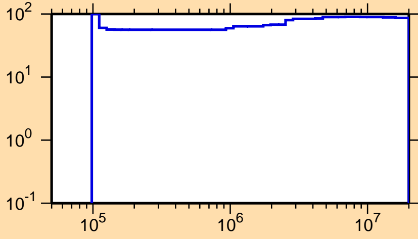
\Delta\sigma/\sigma vs. E for ^{239}\text{Bk}(n,n\text{cont.})
