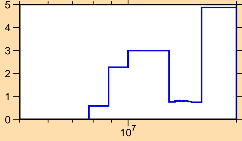
\Delta\sigma/\sigma vs. E for ^{239}\text{Bk}(n,\text{el.})
