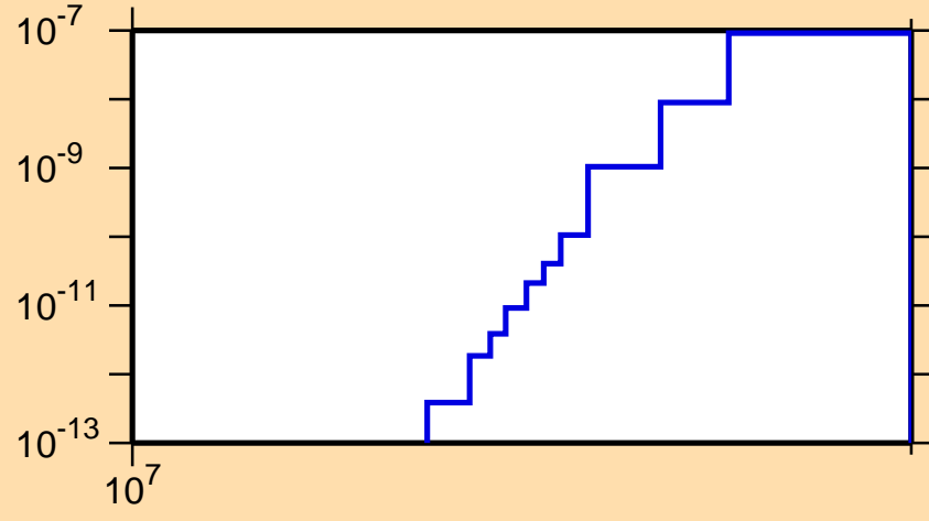
\sigma vs. E for ^{239}\text{Bk}(n,nd)
