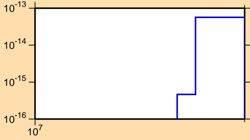
\sigma vs. E for ^{239}\text{Bk} (mt 34)
