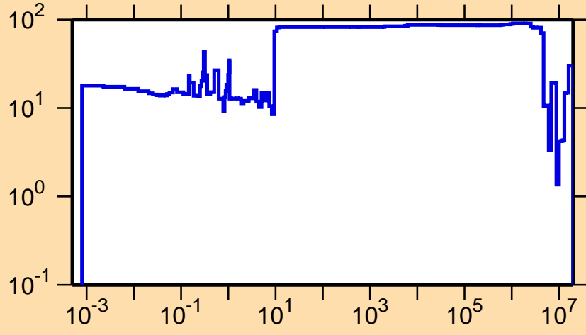
\Delta\sigma/\sigma vs. E for ^{239}\text{Bk}(n,\gamma)
