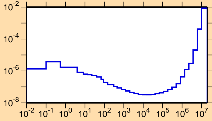
\sigma vs. E for ^{239}\text{Bk}(n,p)
