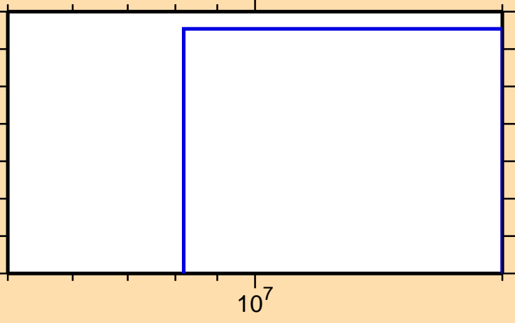
\sigma vs. E for ^{239}\text{Bk}(n,3n)
