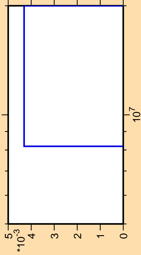
\Delta\sigma/\sigma vs. E for ^{239}\text{Bk} (mt 34)
