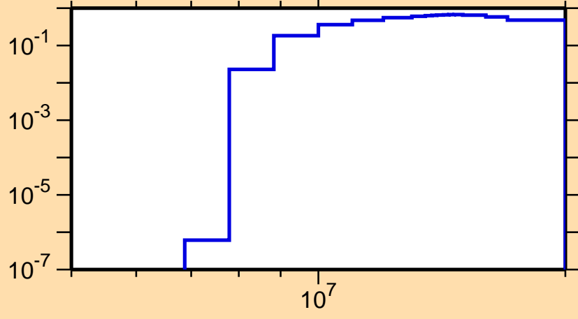
\sigma vs. E for ^{241}\text{Bk}(n,2n)
