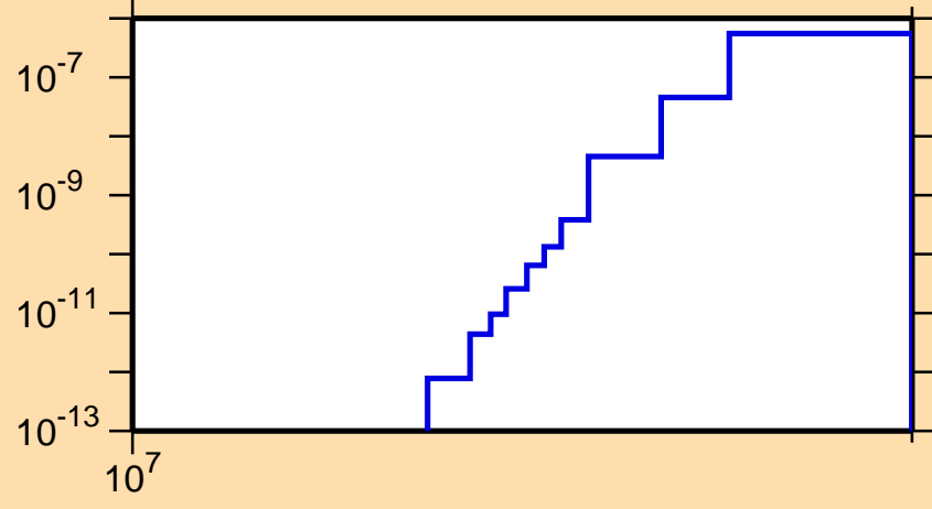
\sigma vs. E for ^{241}\text{Bk}(n,nd)
