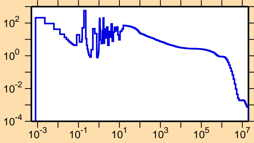
\sigma vs. E for ^{241}\text{Bk}(n,\gamma)
