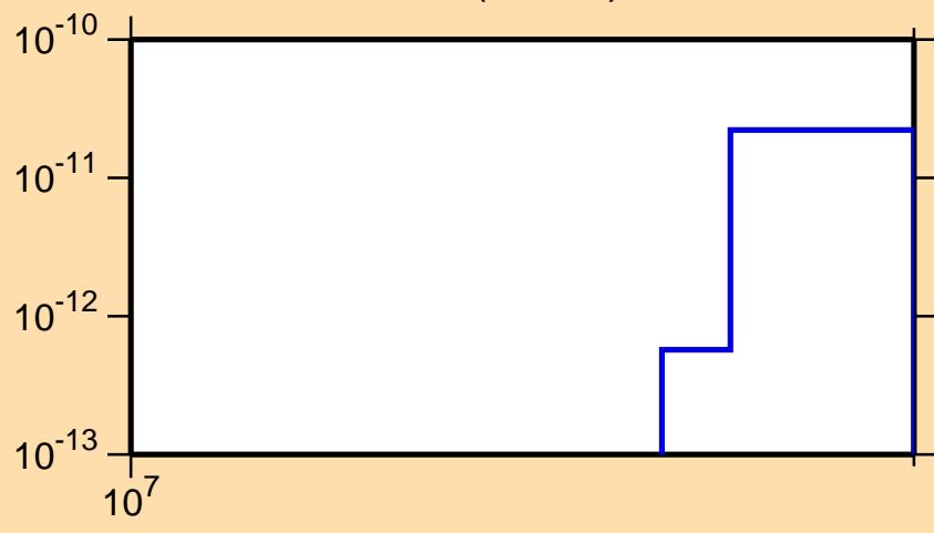
\sigma vs. E for ^{241}\text{Bk}(n,3n\alpha)
