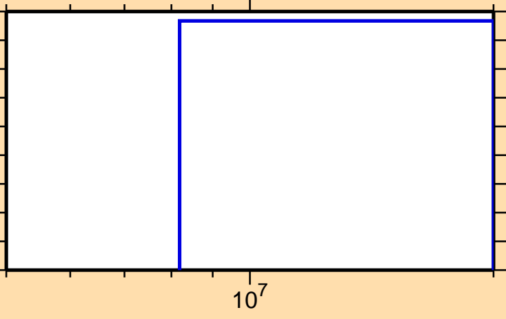
\sigma vs. E for ^{241}\text{Bk}(n,3n)
