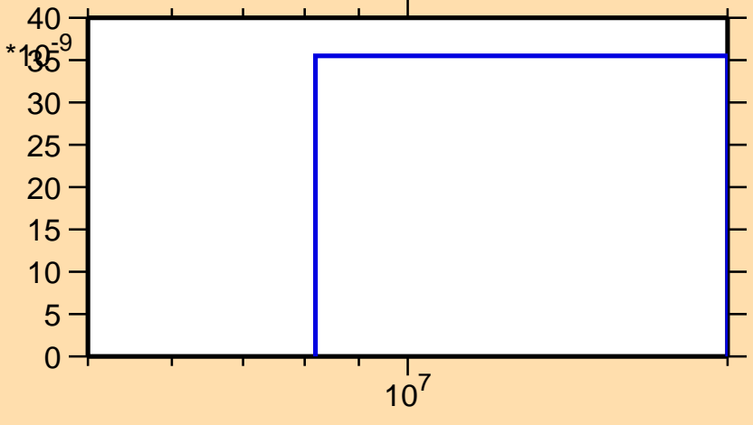
\sigma vs. E for ^{241}\text{Bk}(n,2n\alpha)
