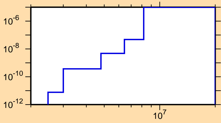
\sigma vs. E for ^{241}\text{Bk}(n,p\alpha)
