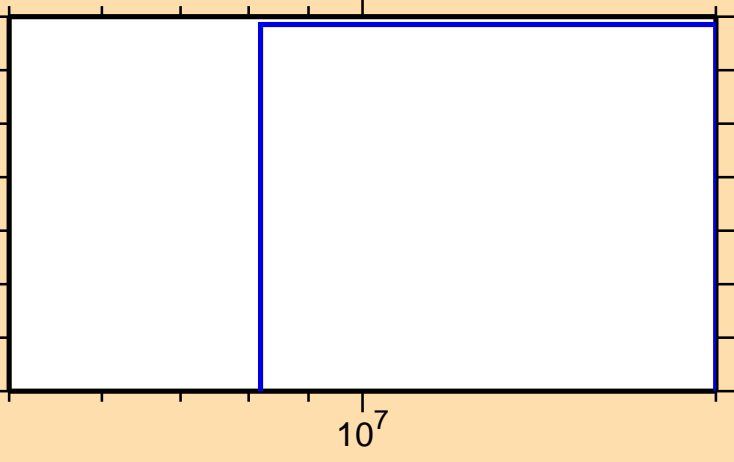
\sigma vs. E for ^{241}\text{Bk}(n,\text{nd})
