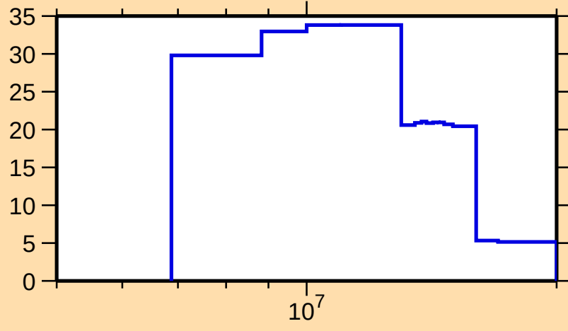
\Delta\sigma/\sigma vs. E for ^{245}\text{Bk}(n,\text{tot.})
