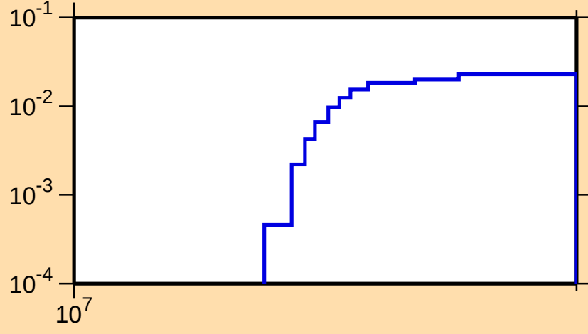
\sigma vs. E for ^{245}\text{Bk}(n,3n)
