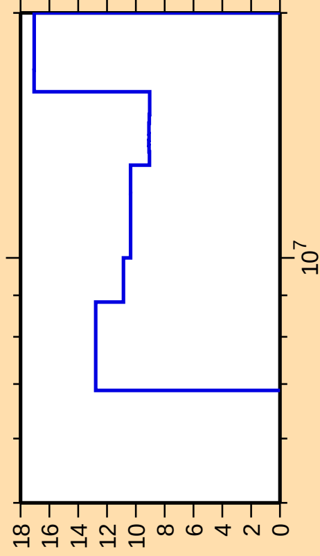
\Delta\sigma/\sigma vs. E for ^{245}\text{Bk}(n,f)
