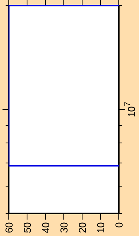
\Delta\sigma/\sigma vs. E for ^{245}\text{Bk}(n,\alpha)
