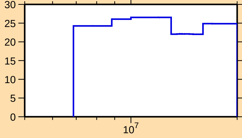
\Delta\sigma/\sigma vs. E for ^{245}\text{Bk}(n,\text{nonel.})
