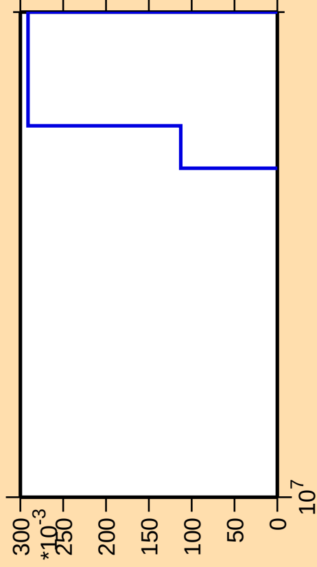
\Delta\sigma/\sigma vs. E for ^{245}\text{Bk}(n,p\alpha)
